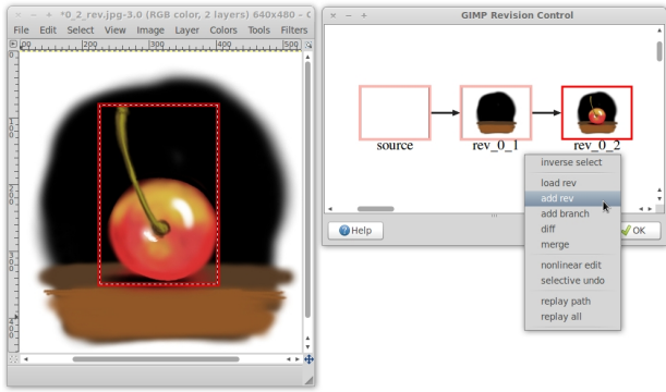
Figure 2: Revision control user interface. Users can perform revision control functions via the right-click menu within the revision control window (right), which also visualizes the revision history through RevG. When a RevG node is selected, its corresponding spatial context will be highlighted via a bounding box in the main GIMP window (left).
