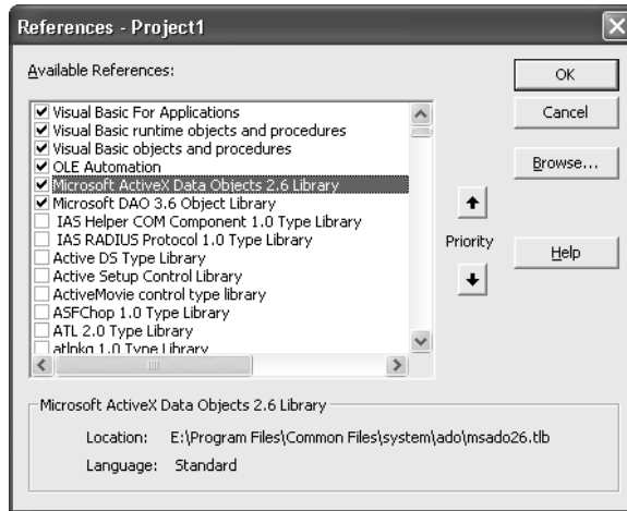
Figure 2-1 ADO 2.6 reference takes precedence over DAO 3.6.
