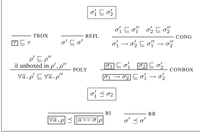
Figure 3: Protected unboxing and boxy instantiation relation
