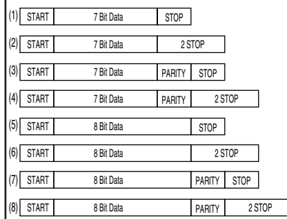
Fig. 2.03. Data, parity, stop bits
