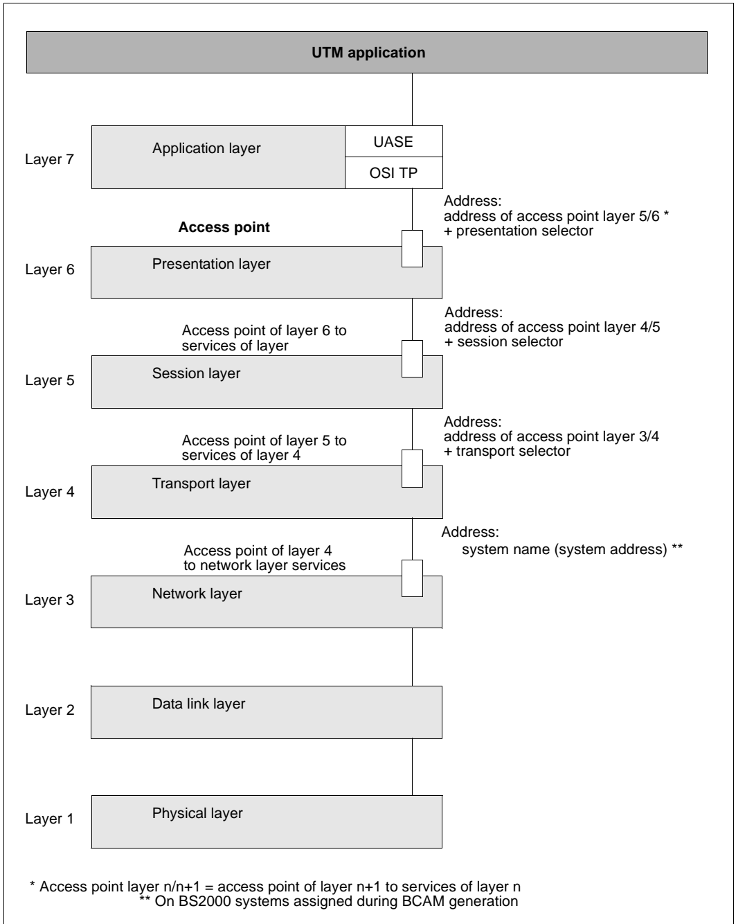
Figure 7: Addresses of the service access points in the OSI reference model
