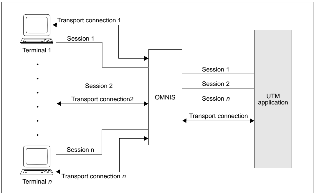
Figure 15: Transport connections and sessions when multiplexing
