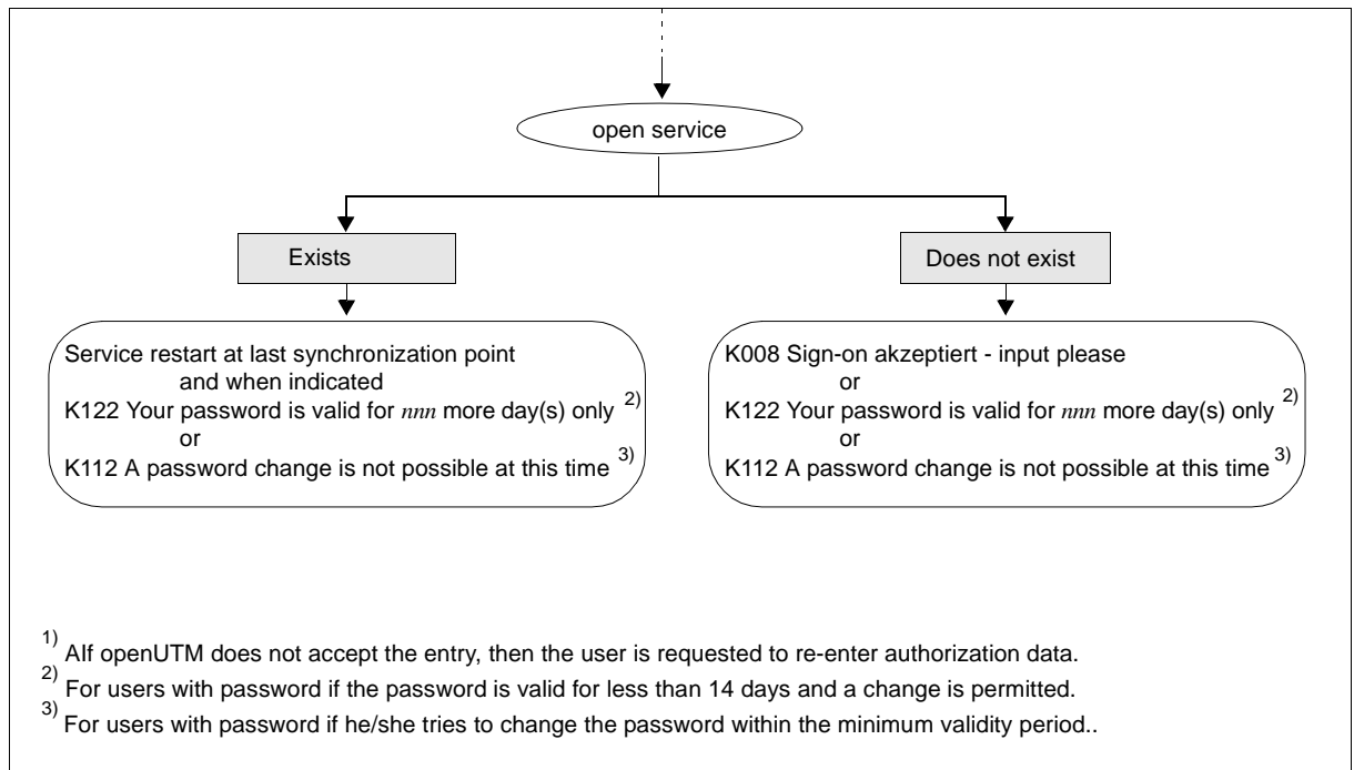
Figure 5: Sign-on check scenarios for applications with logins (part 3)
