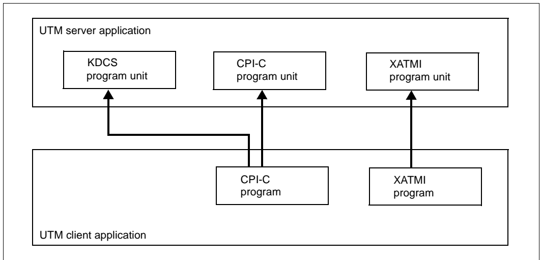
Client/server link
