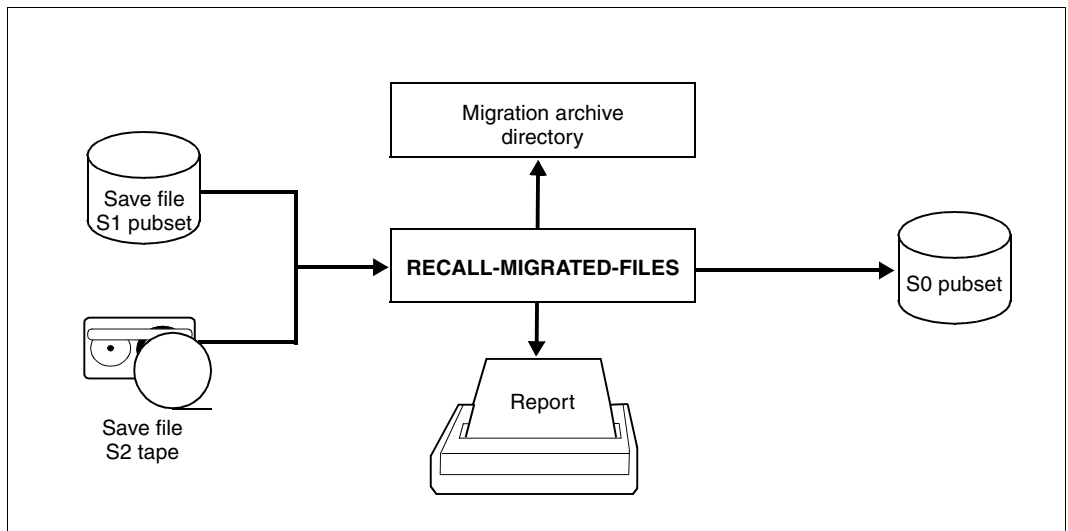
Figure 14: Explicit recall using RECALL-MIGRATED-FILES
