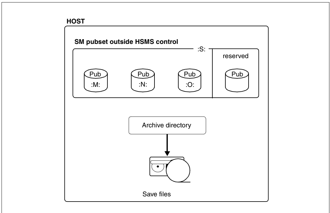
Figure 22: SM pubset outside HSMS control
