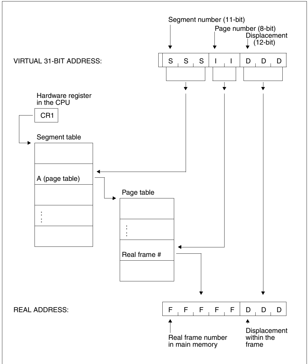
Figure 5: Address conversion for a 31-bit address
