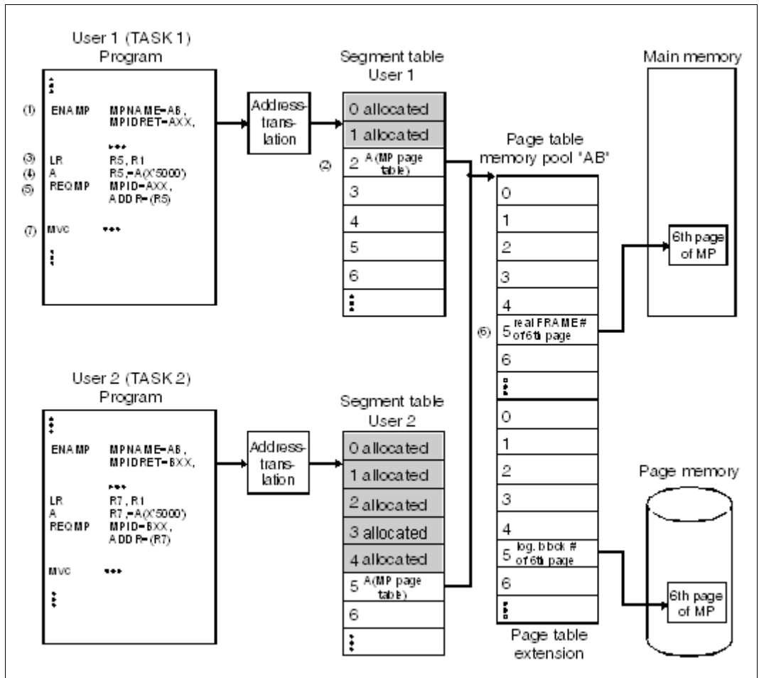
Figure 6: Establishing a connection to and accessing a memory pool page (/390 servers)
