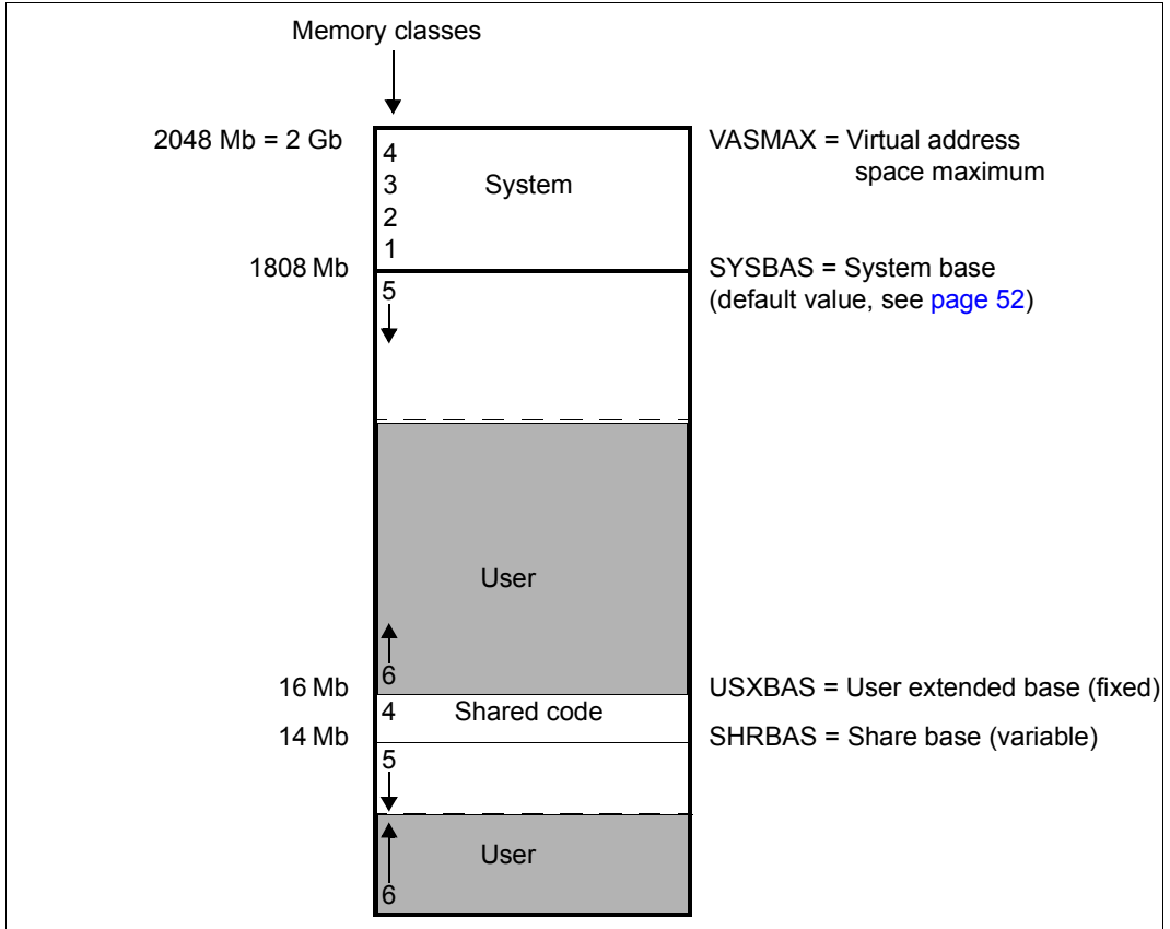
Figure 4: Structure of virtual address space (/390 servers)
