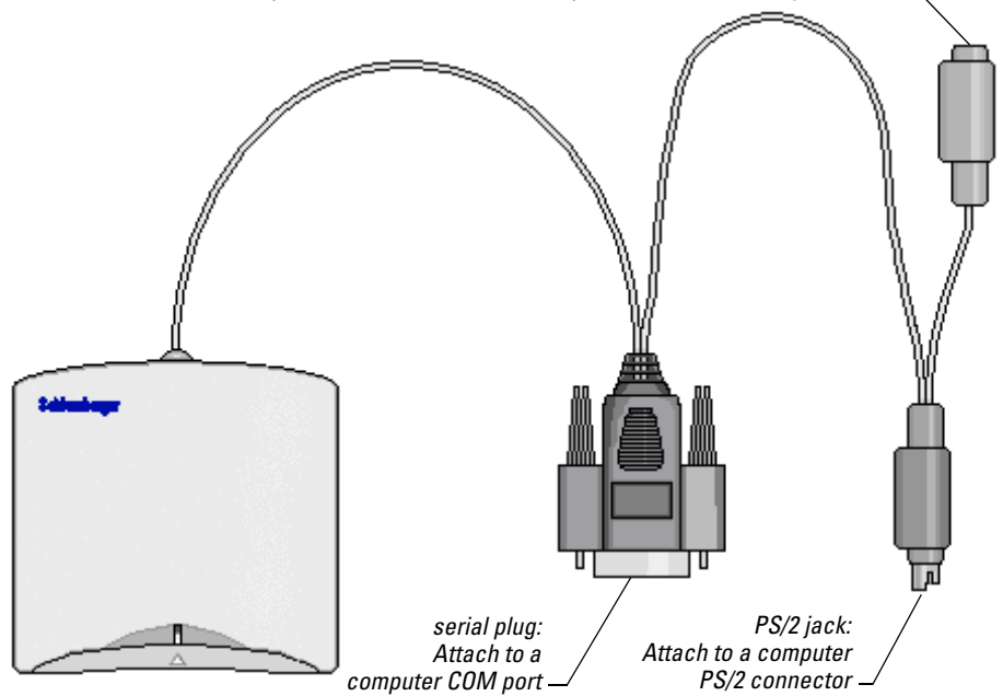
Reader Connectors
