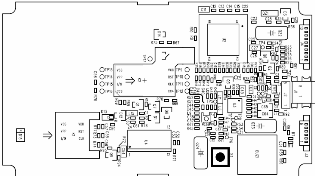
Figure 31 – Push button PCB location (S1)
