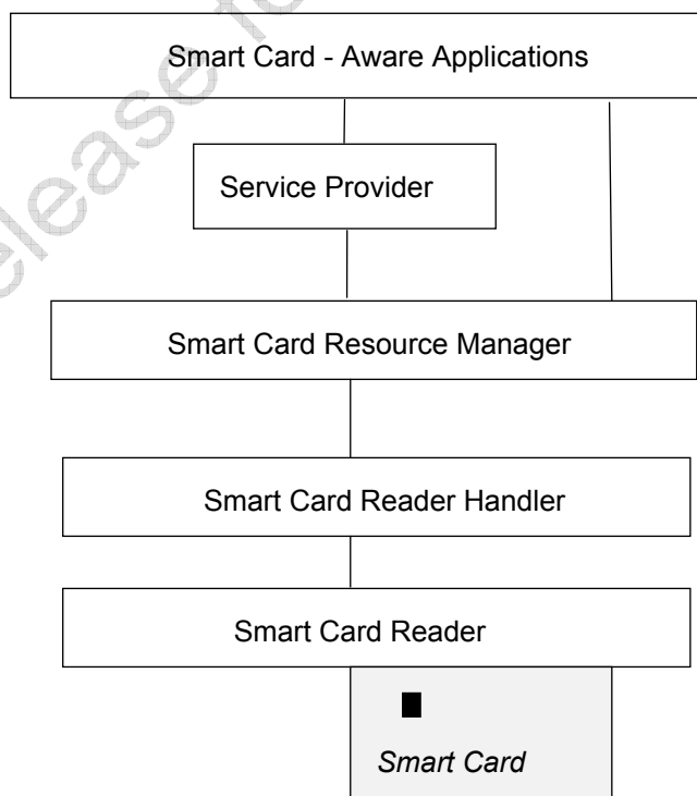
Figure 23 – PC/SC Architecture
