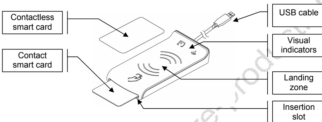
Figure 1 – Prox-DU view
