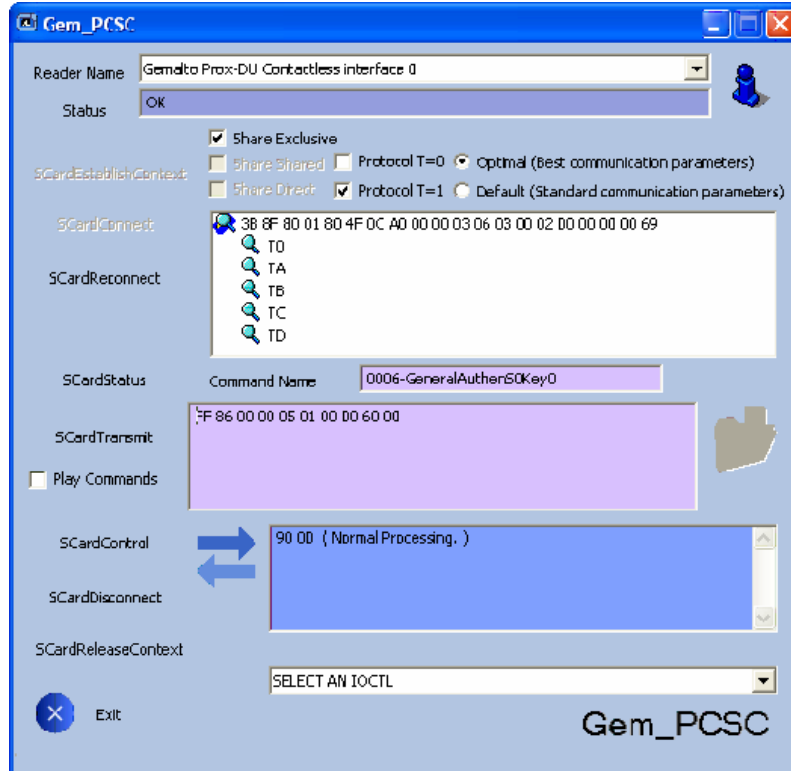
Figure 24 – Gem_PCSC window
