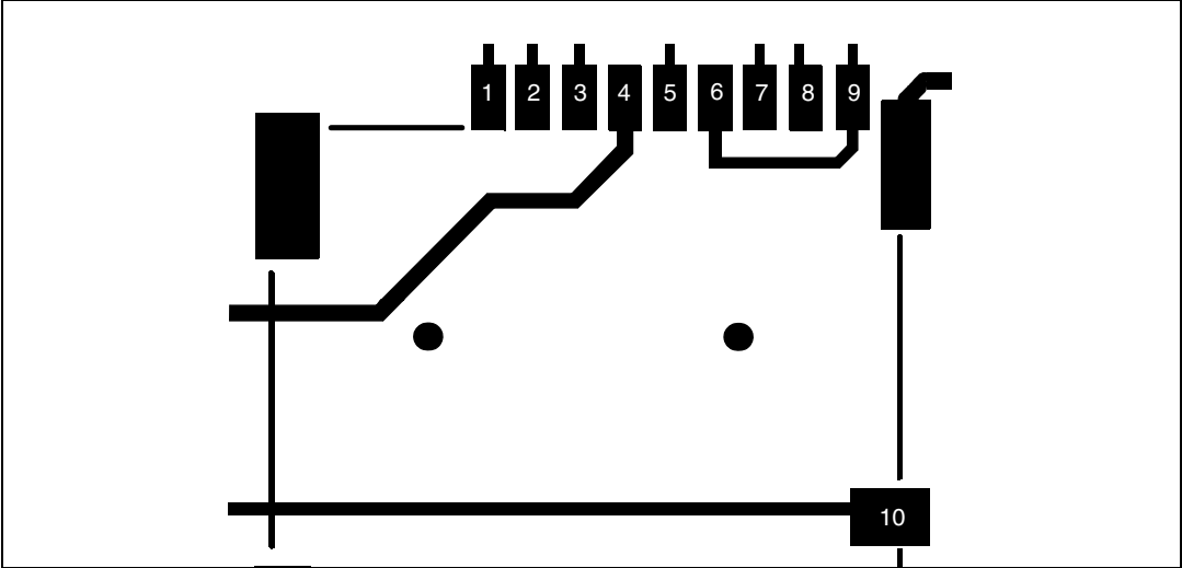
Figure 19. MicroSD card connector (CN16) pinout
