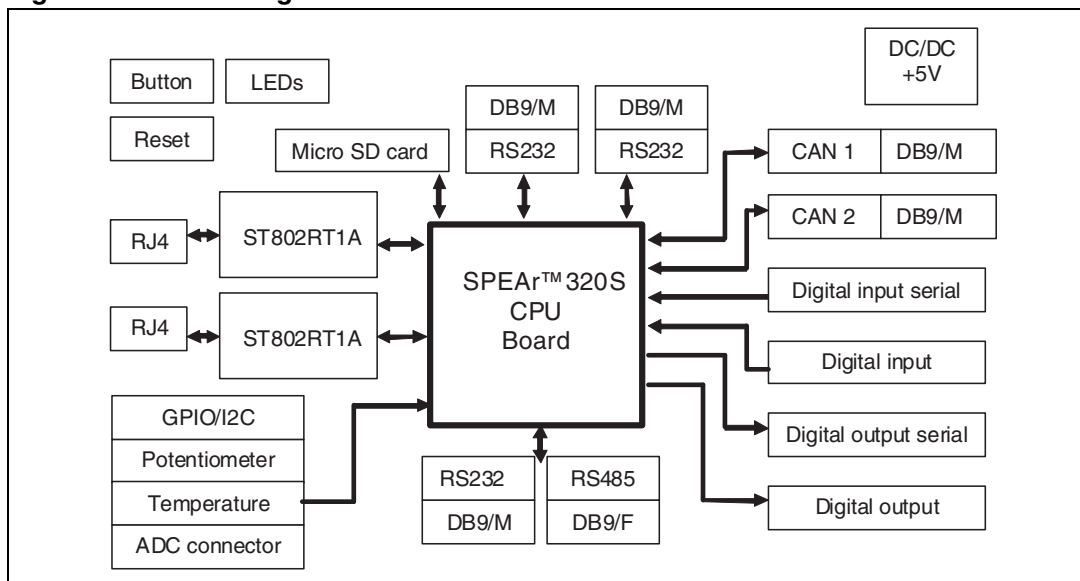
Figure 2. Block diagram
