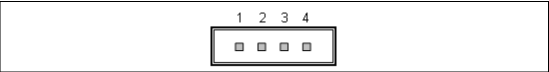
Figure 15. RS-485 header connector CN12 pinout
