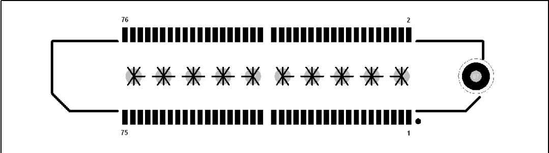
Figure 22. 86-pin connectors (J1 and J2) pinout
