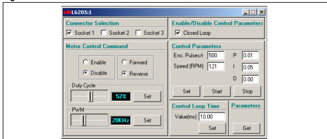
Figure 9. 6205 window
