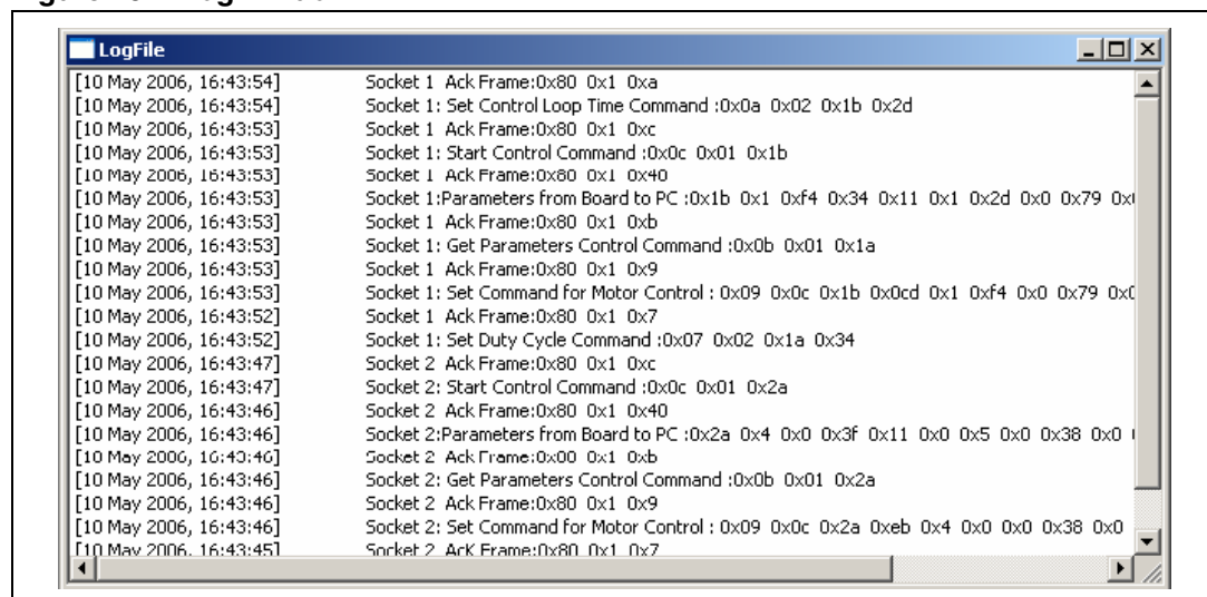
Figure 10. Log window
