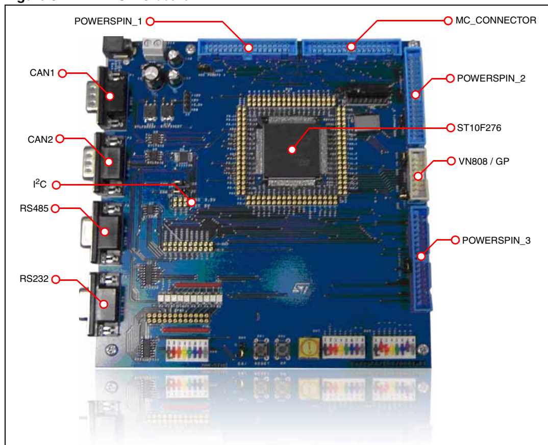
Figure 3. MDK-ST10 board
