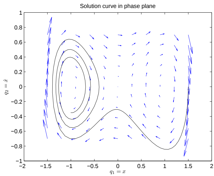
Figure 5.6: Trajectory of Duffing equation in Phase plane
