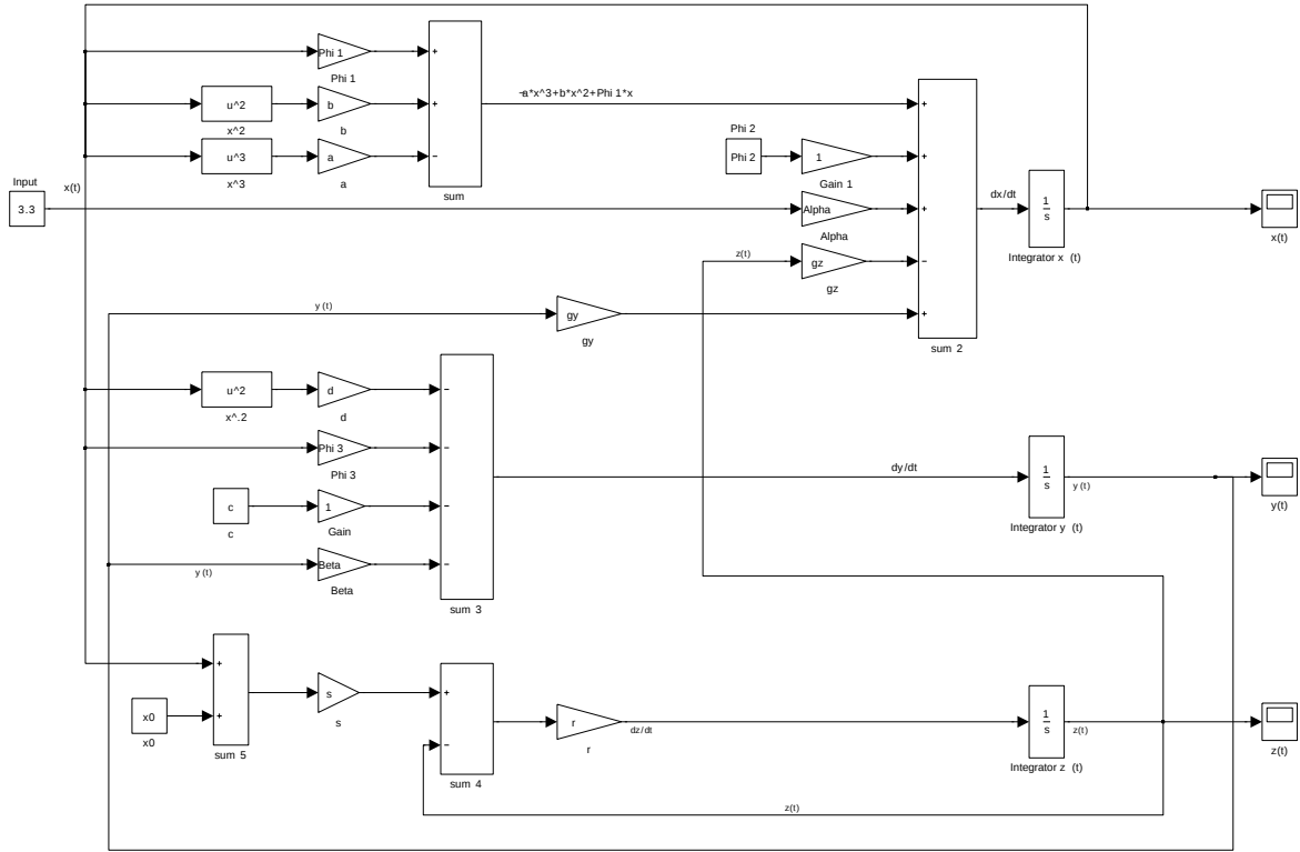
Figure 7.1: Simulink scheme of neuron model
