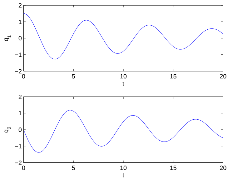
Figure 5.2: Trajectory in time
