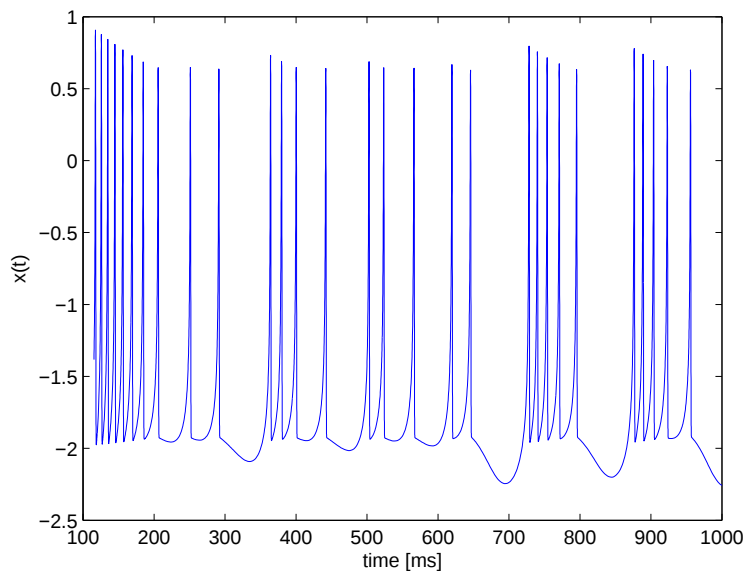
Figure 7.2: Time trajectory of neuron model
