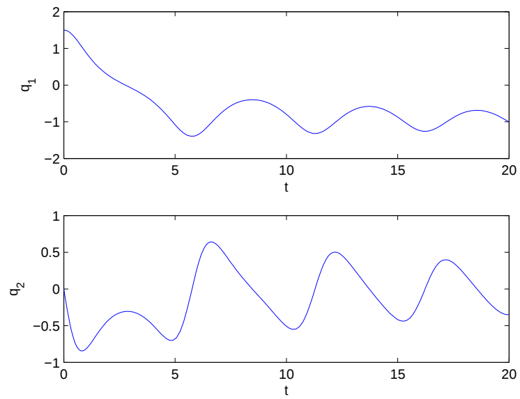
Figure 5.5: Time trajectory of Duffing equation
