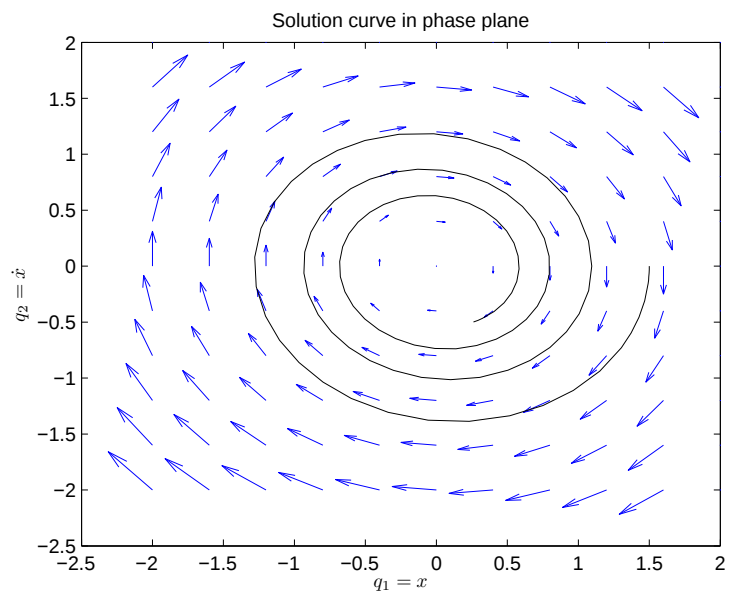
Figure 5.3: Trajectory in phase plane
