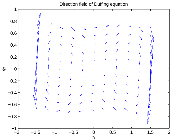
Figure 5.4: Direction field of Duffing equation
