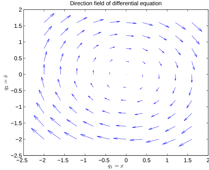
Figure 5.1: Direction field
