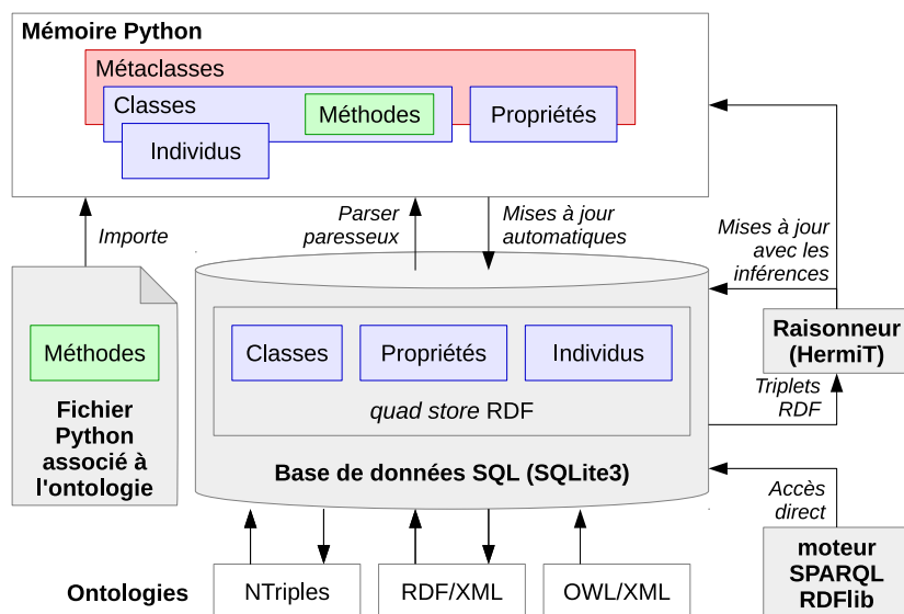
FIGURE 2.8 – Architecture du module Owlready (version 2).
