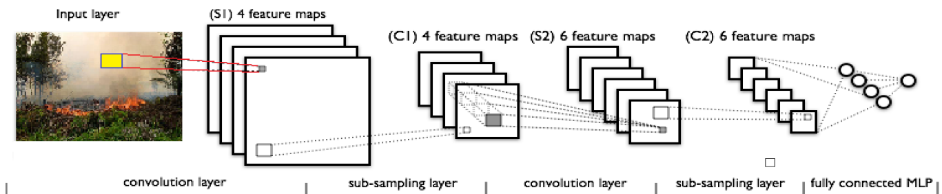
Fig. 2. CNN layers
