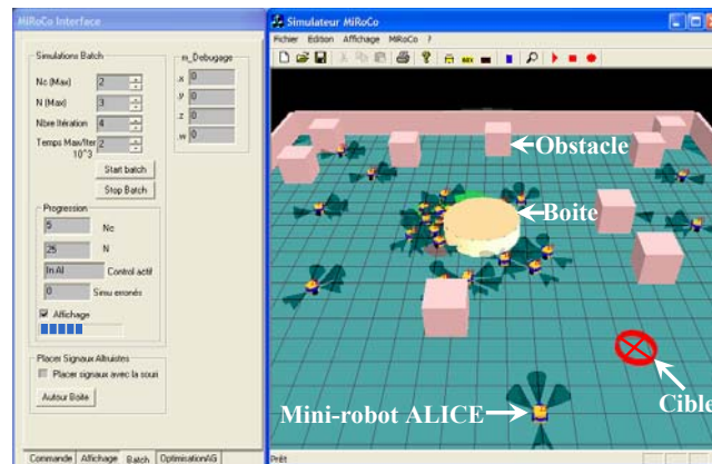
Figure 3. Simulateur MiRoCo “MiniRobotique Collective”
