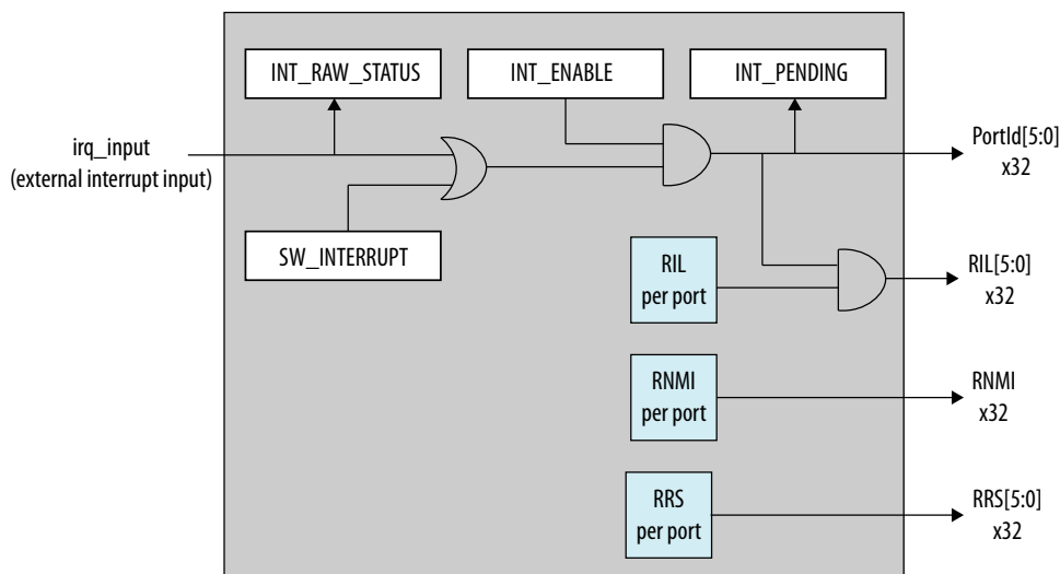
Figure 113. Interrupt Request Block
