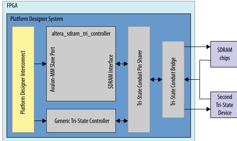
Figure 103. Shared-Bus System
