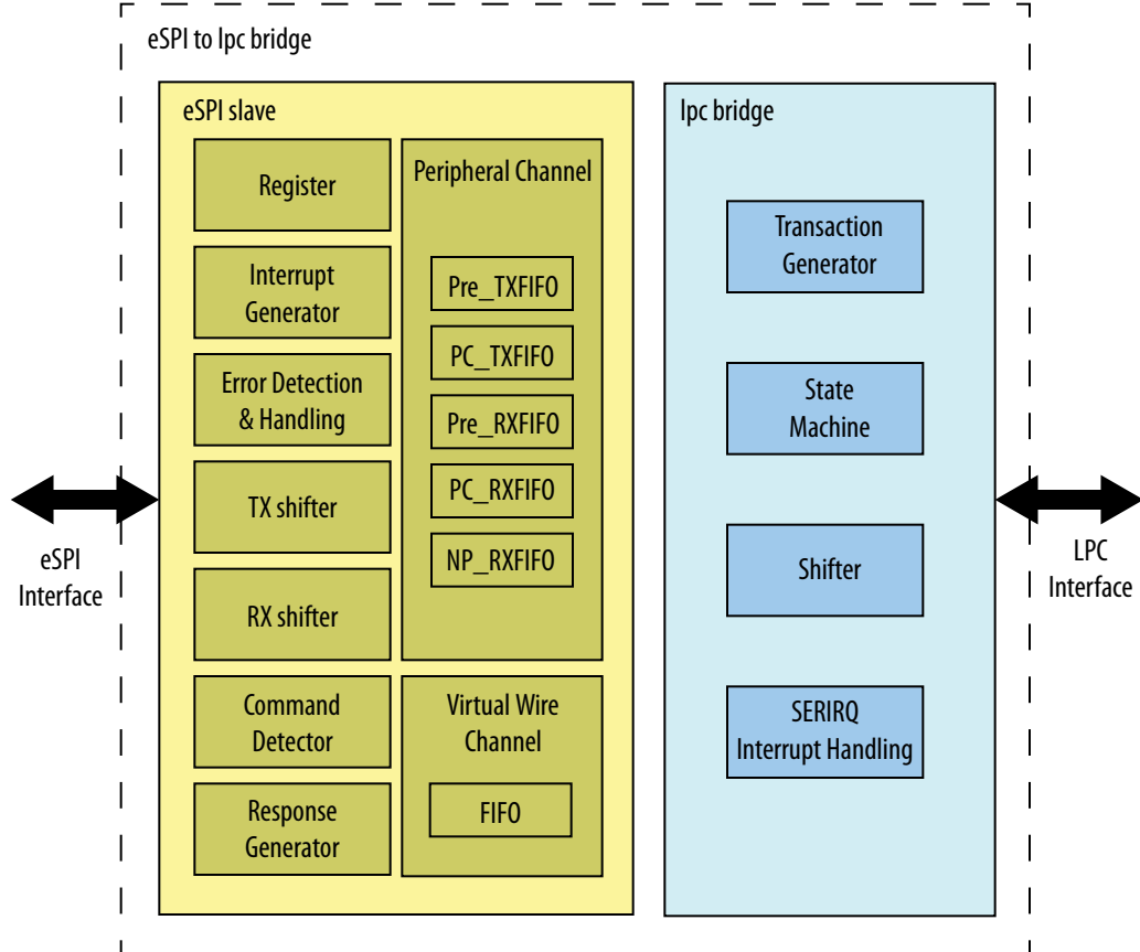
Figure 26. Block Diagram
