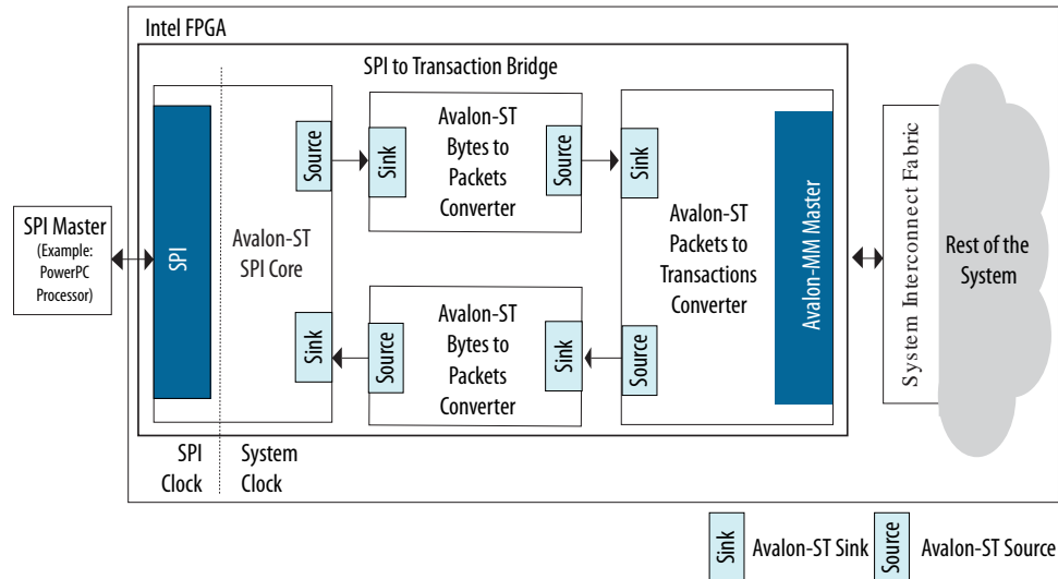
Figure 15. System with a SPI Slave to Avalon Master Bridge Core
