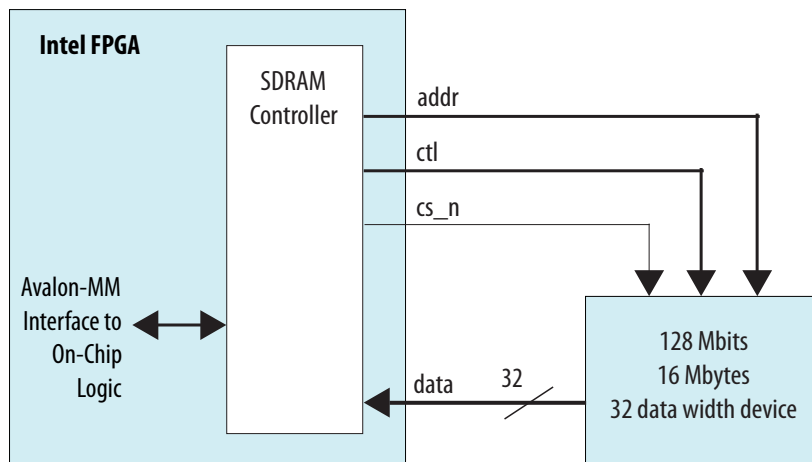
Figure 97. Single 128-Mbit SDRAM Chip with 32-Bit Data
