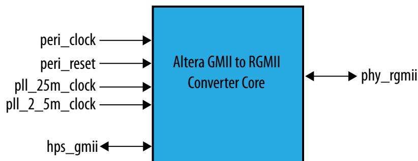
Figure 138. Intel FPGA GMII to RGMII Converter Core Top Level Interfaces
