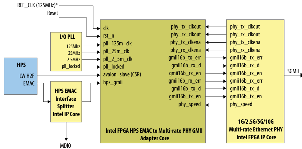
Figure 153. Block Diagram
