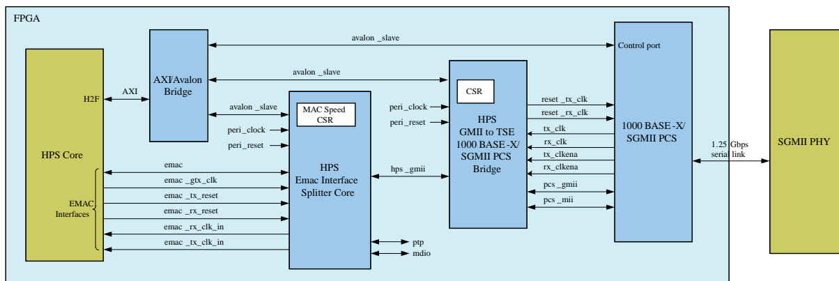
Figure 148. Intel FPGA HPS GMII to TSE 1000BASE-X/SGMII PCS Bridge Core Block Diagram
