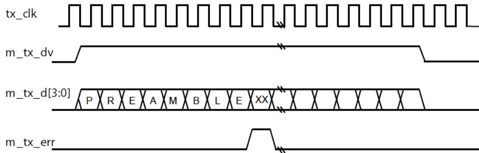
Figure 146. TX Frame with Error Signal
