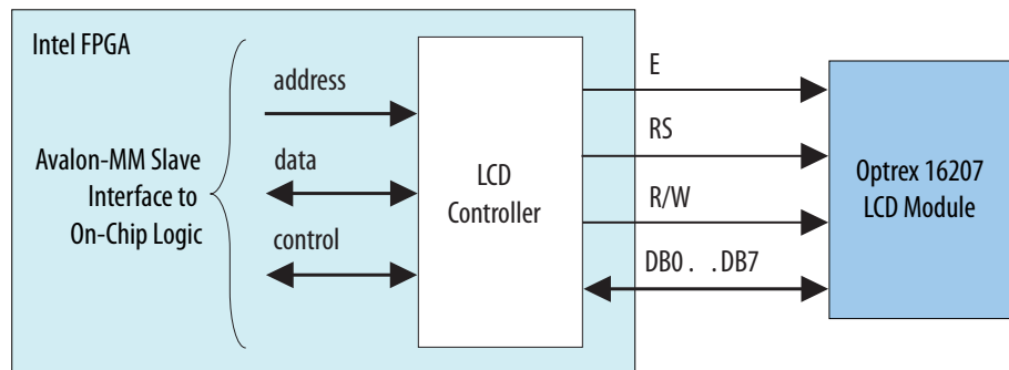
Figure 78. LCD Controller Block Diagram
