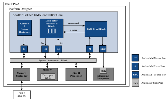
Figure 94. Example of Memory-to-Stream Configuration
