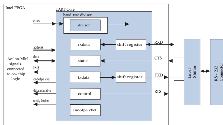
Figure 39. Block Diagram of the UART Core in a Typical System
