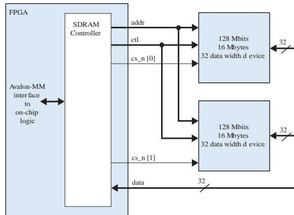
Figure 99. Two 128-Mbit SDRAM Chips Each with 32-Bit Data
