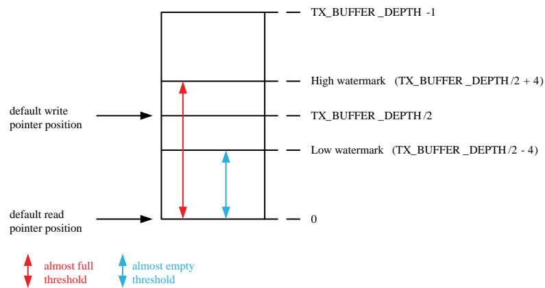
Figure 151. Elastic Buffer Watermark Level
