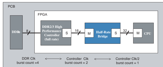
Figure 136. Platform Designer Memory System Using a DDR Memory Half-Rate Bridge
