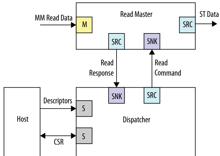
Figure 85. mSGDMA Module Configuration with Support for Memory-Mapped Streaming Reads to the Avalon-ST data bus
