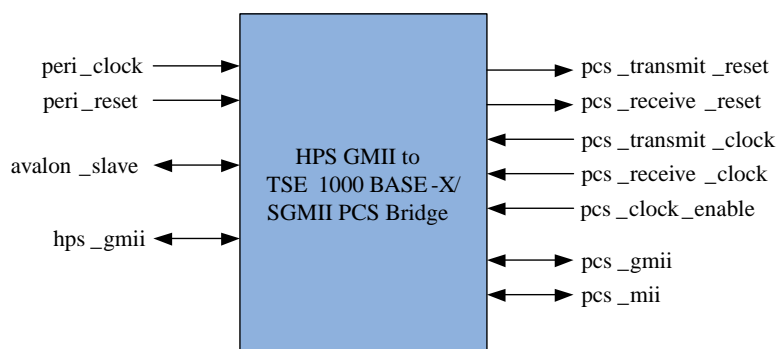
Figure 152. Intel FPGA HPS GMII to TSE 1000BASE-X/SGMII PCS Bridge Top Level Interfaces
