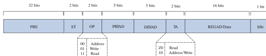
Figure 30. MDIO Frame Format (Clause 45)
