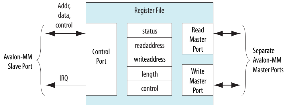
Figure 83. DMA Controller Block Diagram
