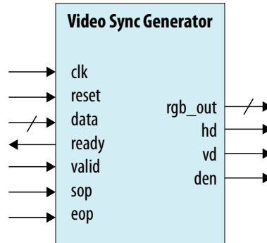
Figure 105. Video Sync Generator Block Diagram
