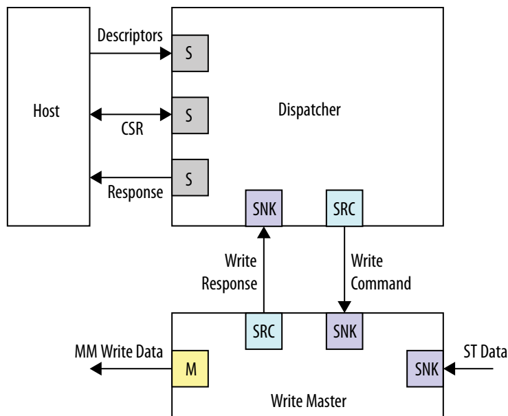
Figure 86. mSGDMA Module Configuration with Support for Avalon-ST Data Write Streaming to the Memory-Mapped Bus
