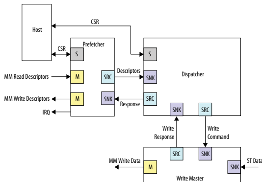
Figure 90. Streaming to Memory-Mapped Configuration with Prefetcher Enabled
