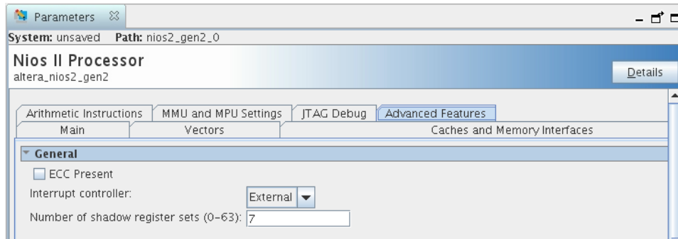
Figure 115. Nios II Processor with EIC Interface
