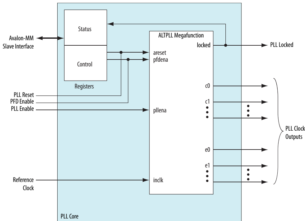
Figure 82. PLL Core Block Diagram
