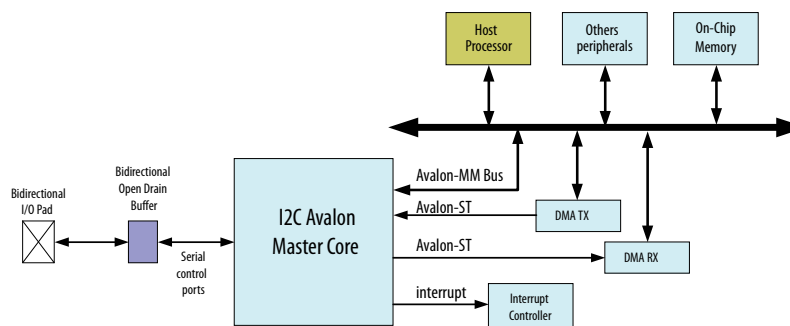
Figure 46. Intel FPGA Avalon I 2 C Master Core with DMA
