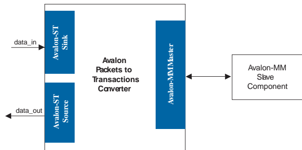
Figure 126. Avalon Packets to Transactions Converter Core
