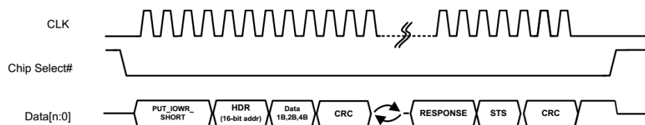
Figure 24. eSPI Master Initiated Short IO Write Transaction
