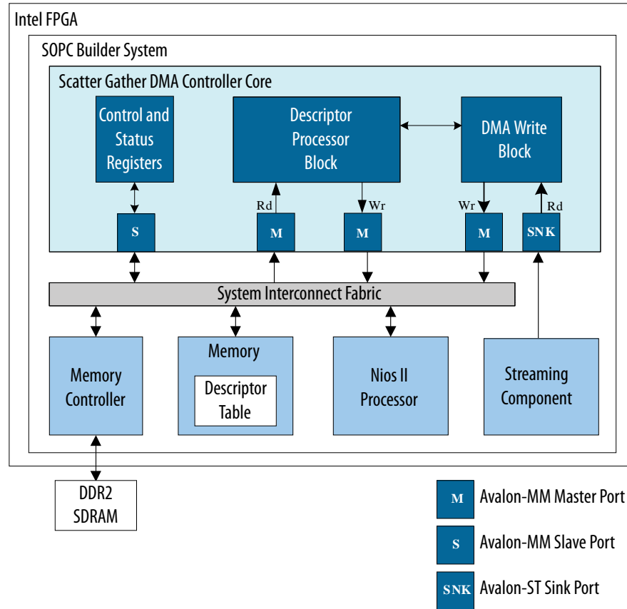
Figure 91. SG-DMA Controller Core with Streaming Peripheral and External Memory
