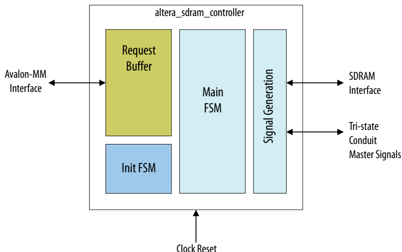
Figure 102. Tri-State SDRAM Block Diagram
