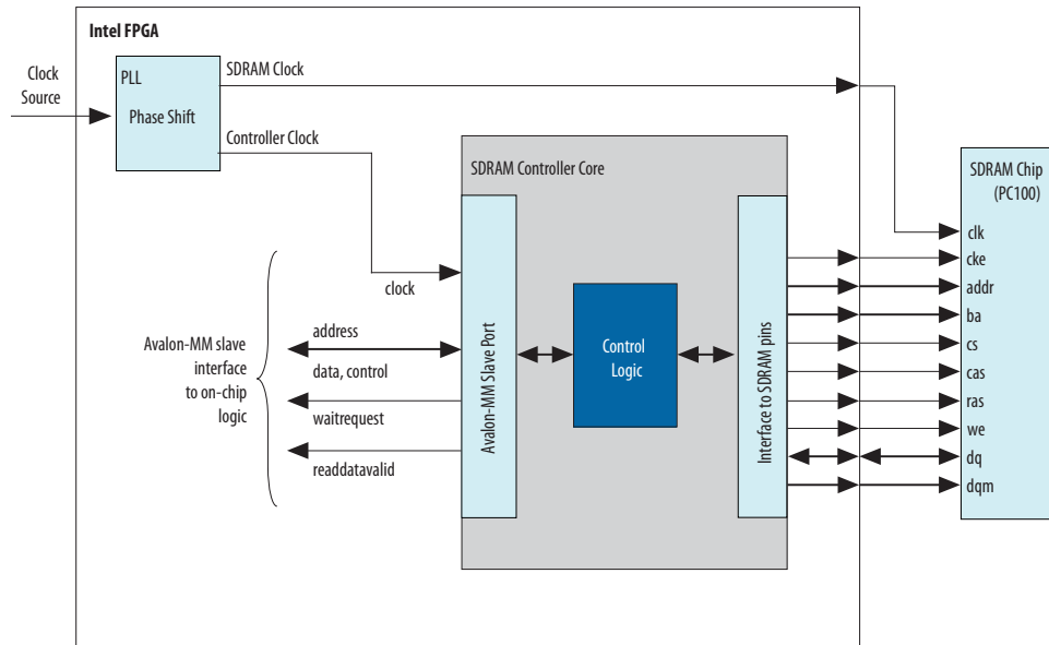
Figure 96. SDRAM Controller with Avalon Interface Block Diagram
