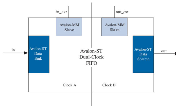
Figure 4. Avalon-ST Dual Clock FIFO Core
