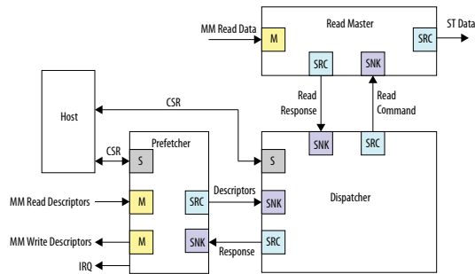
Figure 89. Memory-Mapped to Streaming Configuration with Prefetcher Enabled
