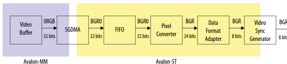
Figure 104. Typical Placement in a System
