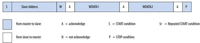
Figure 47. Master Transmitter Writes 2 Bytes to Slave Receiver
