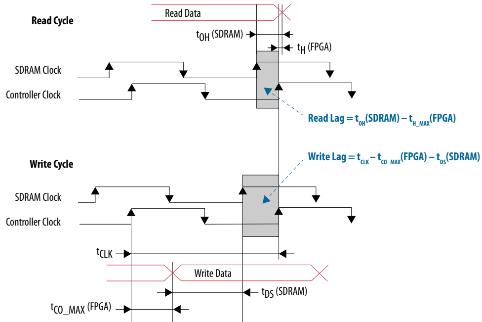
Figure 100. Calculating the Maximum SDRAM Clock Lag
