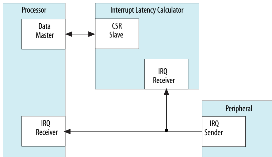
Figure 109. Usage model of Interrupt Latency Calculator
