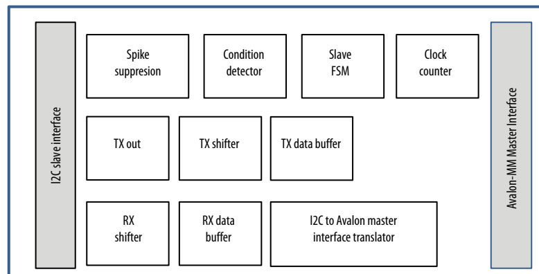
Figure 55. Intel FPGA I 2 C to Avalon-MM Master Bridge Block Diagram
