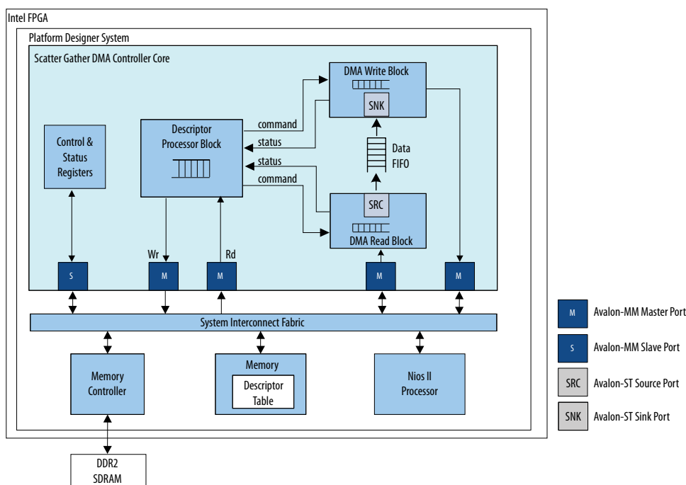
Figure 93. Example of Memory-to-Memory Configuration
