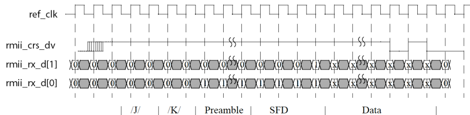
Figure 147. RMII Receive Transfer
