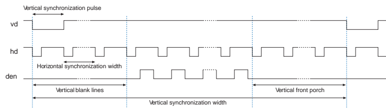
Figure 108. Vertical Synchronization Timing—8 Bits DataWidth and 3 bits Per Pixel / 24 Bits DataWidth and 1 Beat Per Pixel
