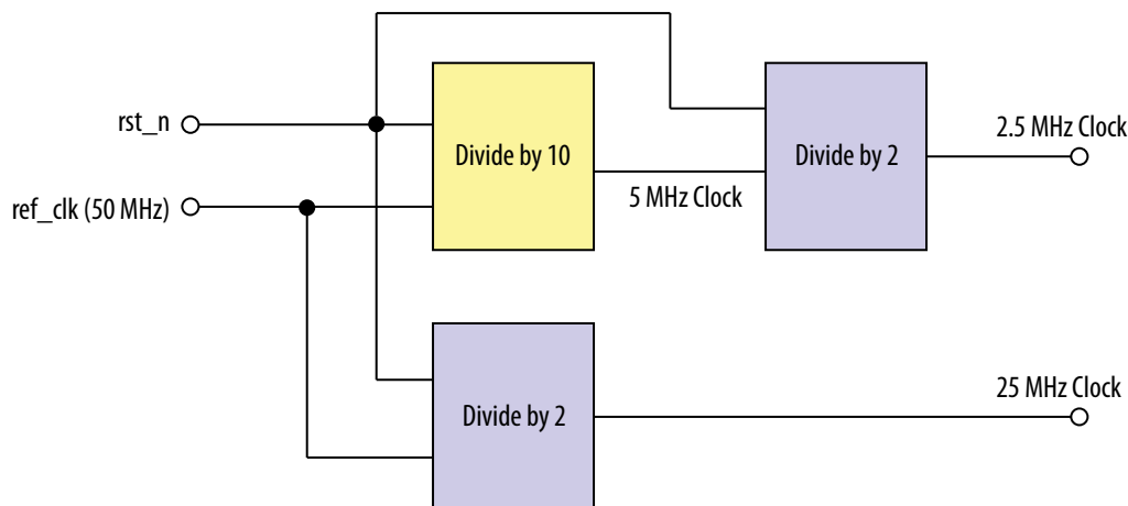
Figure 144. Clocking Scheme
