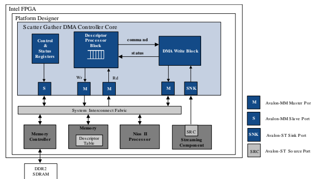
Figure 95. Example of Stream-to-Memory Configuration
