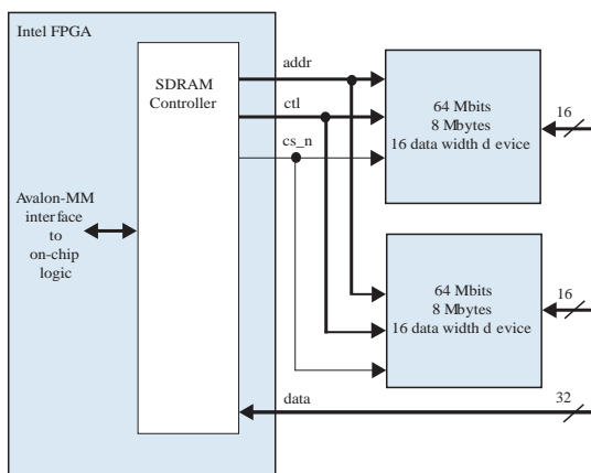
Figure 98. Two 64-Mbit SDRAM Chips Each with 16-Bit Data
