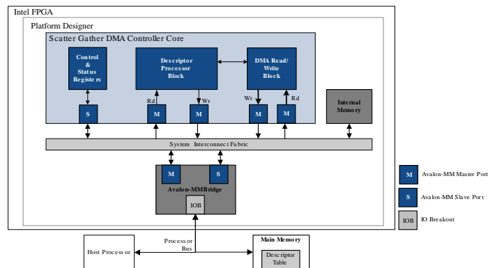
Figure 92. SG-DMA Controller Core with Internal and External Memory
