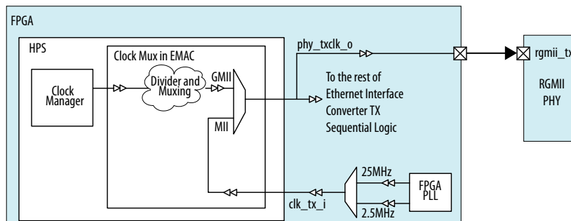
Figure 141. Transmit Clocking Scheme
