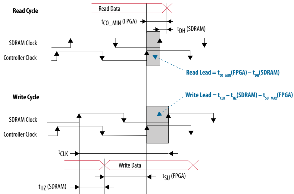
Figure 101. Calculating the Maximum SDRAM Clock Lead
