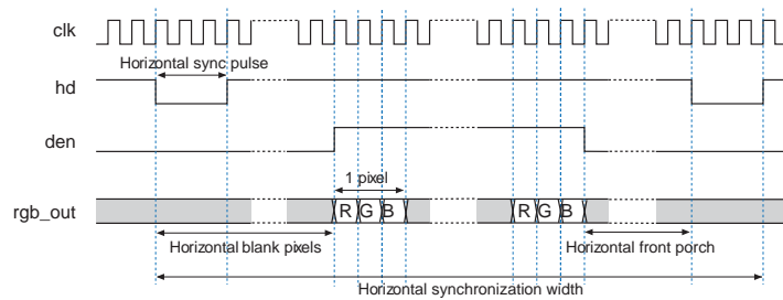
Figure 106. Horizontal Synchronization Timing—8 Bits DataWidth and 3 bits Per Pixel
