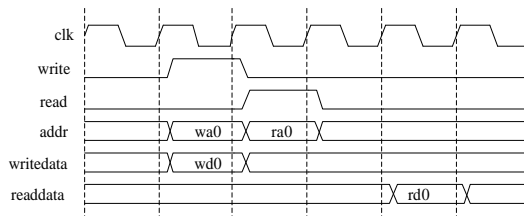
Figure 53. Write and Read Timing of Avalon-MM Slave Interface
