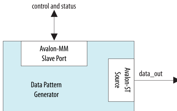
Figure 123. Data Pattern Generator Core Block Diagram
