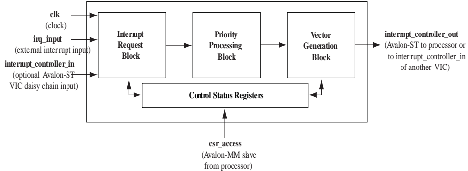
Figure 112. VIC Block Diagram
