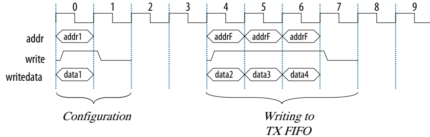
Figure 36. Writing to UART over Avalon-MM
