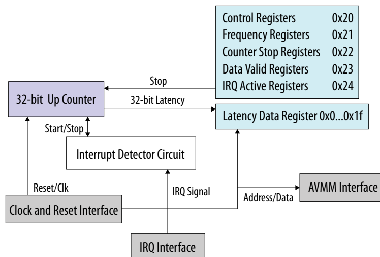
Figure 110. Interrupt Latency Calculator Architecture
