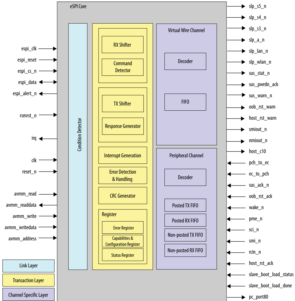
Figure 21. Block Diagram
