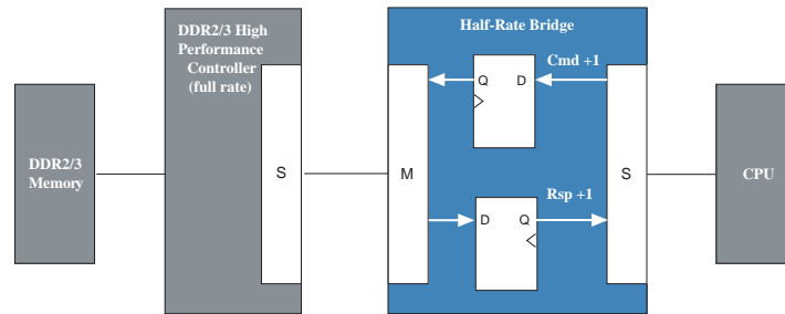
Figure 137. Avalon-MM DDR Memory Half-Rate Bridge Block Diagram
