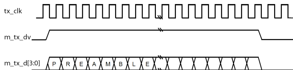
Figure 145. MII TX Frame
