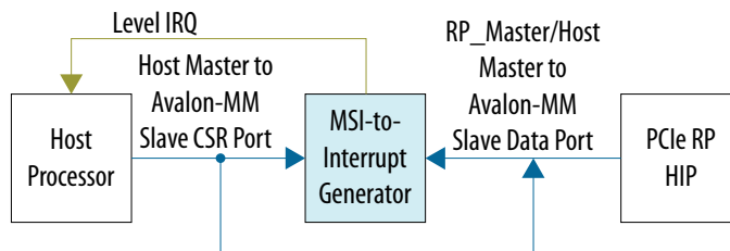
Figure 155. MSI-to-GIC Generator in PCIe RP system
