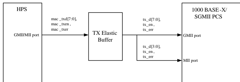
Figure 149. Transmit Data Path
