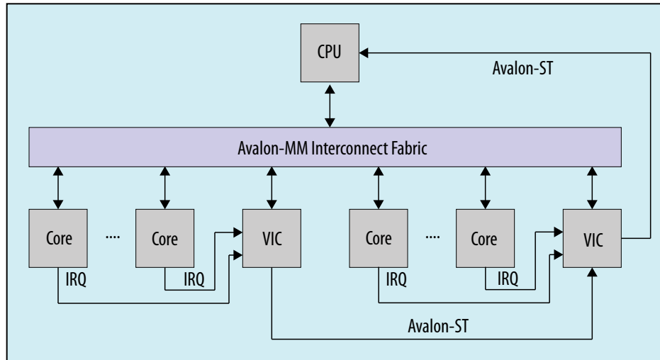
Figure 111. Sample System Layout
