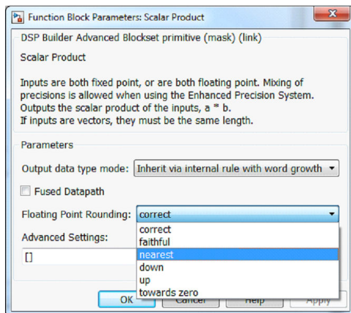
Figure 88. Floating-Point Rounding
