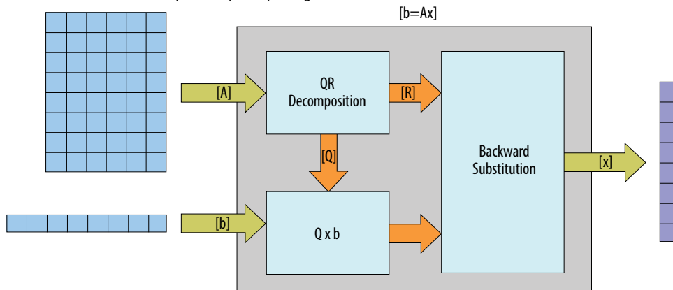
Figure 72. QRD Solver
