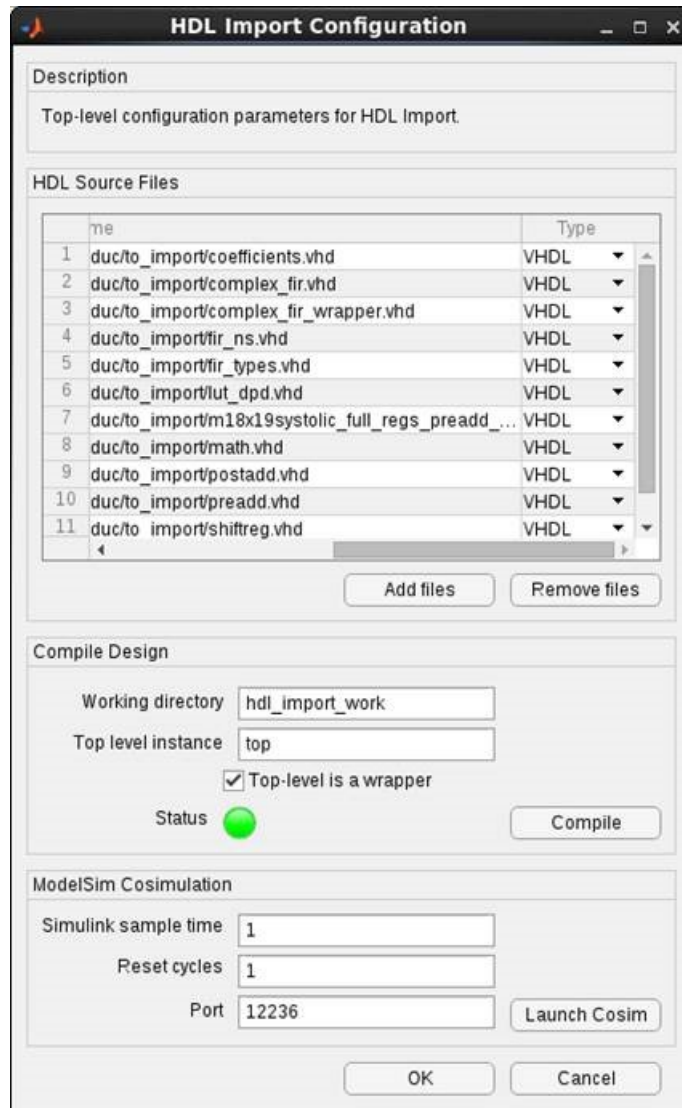
Figure 64. HDL Import Configuration
