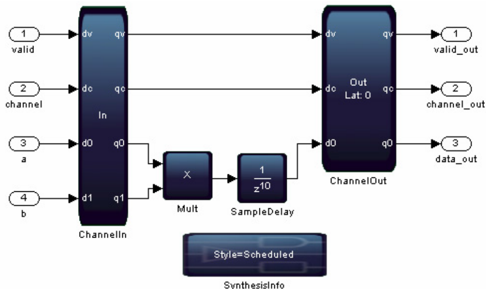
Figure 73. Latency Example with a User-Specified Delay
