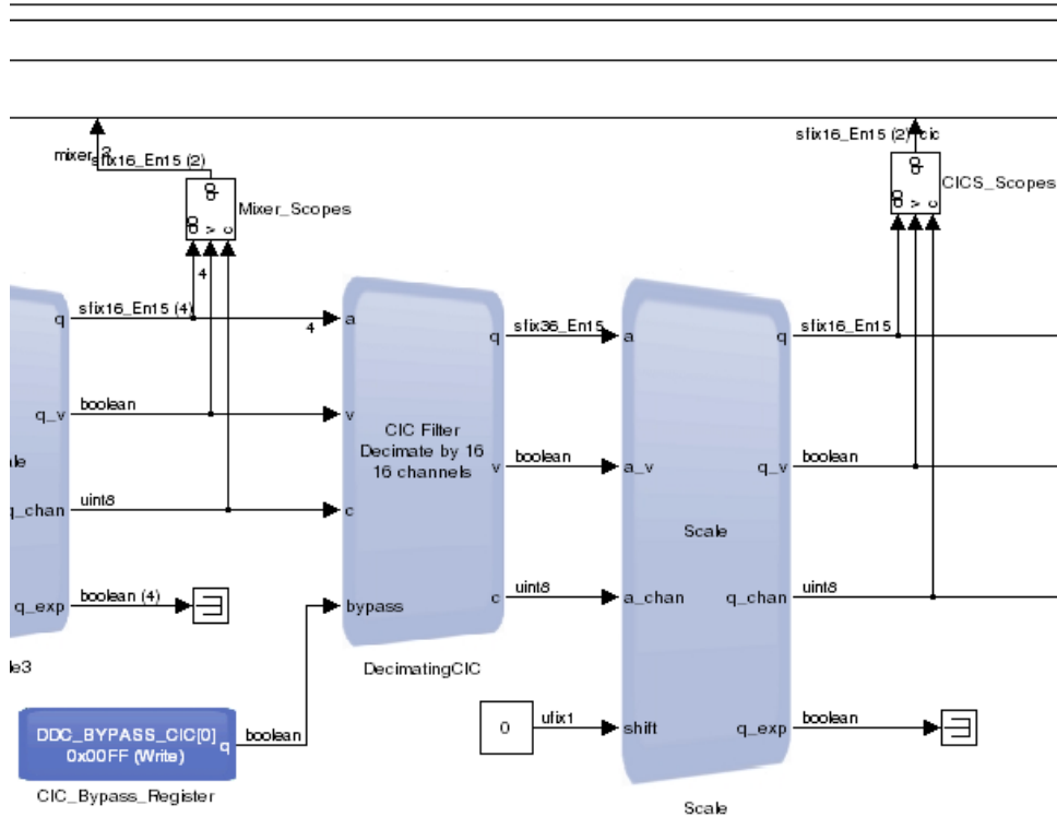
Figure 38. DDCChip Datapath (DecimatingCIC and Scale Blocks)
