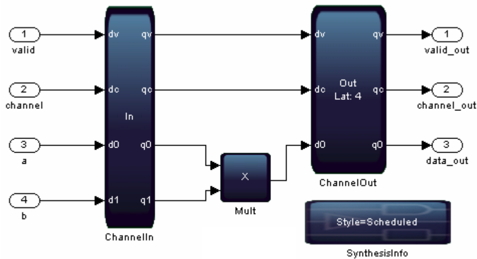
Figure 75. Latency Example without a User-Specified Delay
