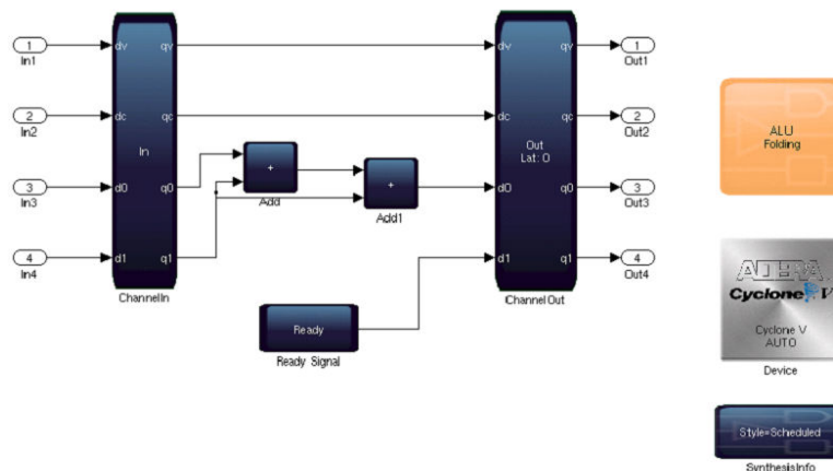
Figure 87. Connecting Ready Block
