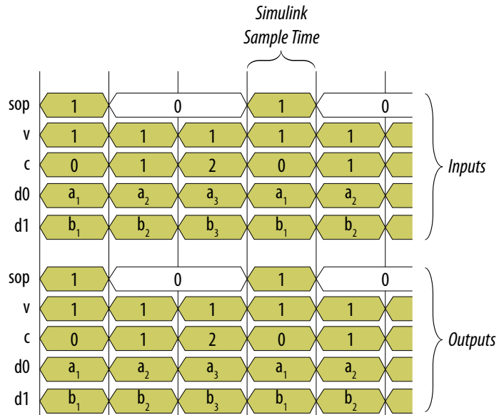
Figure 81. Multichannel Data Rate Simulation with no Register Outputs
