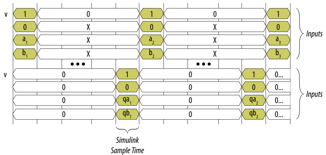
Figure 82. Single Channel Clock Rate Simulation with no Register Outputs
