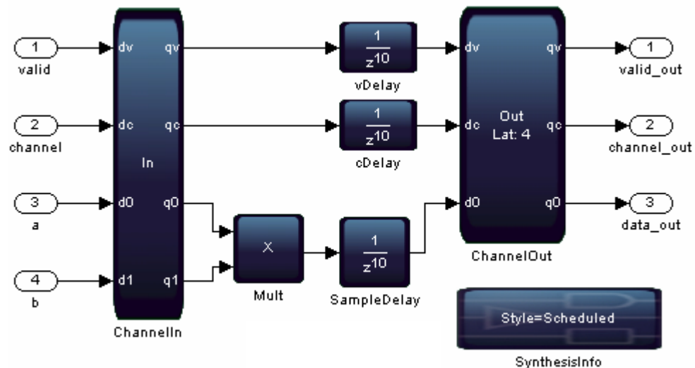
Figure 76. Latency Example with Consistent Delays
