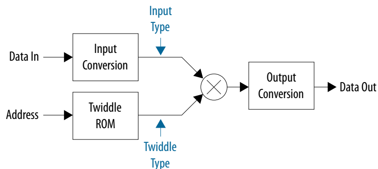
Figure 95. Pruning and Twiddle for FFT Blocks
