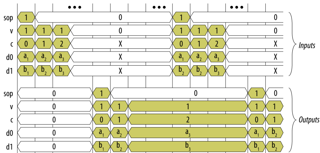
Figure 85. Multichannel Clock Rate Simulation with Register Outputs
