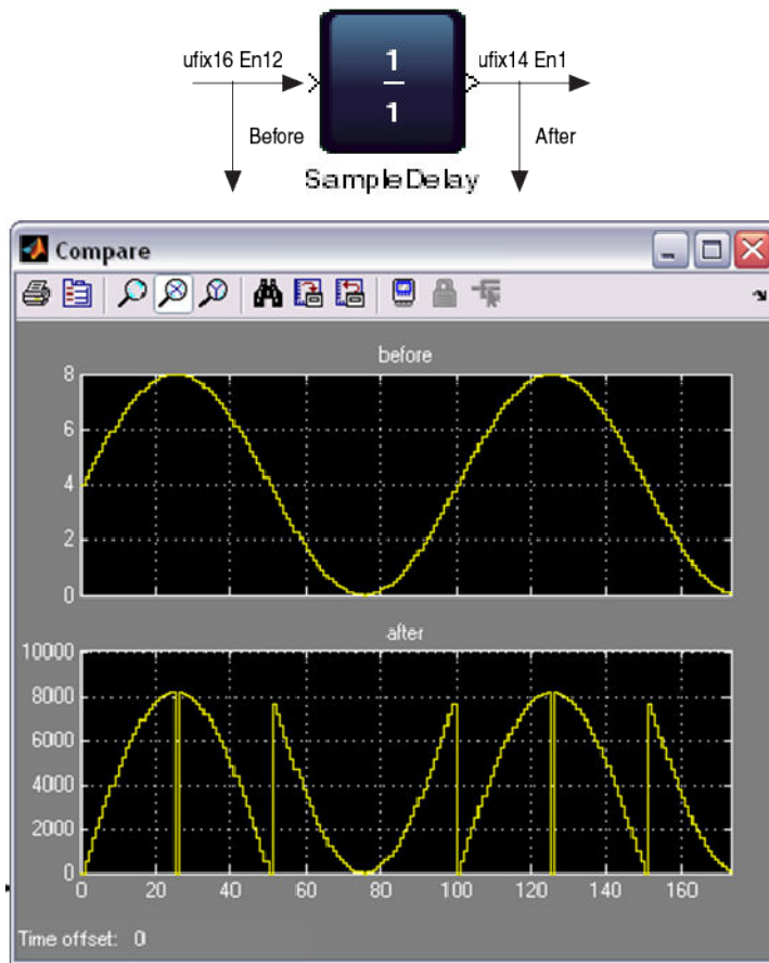
Figure 24. SampleDelay Block and Reducing Bit Width
