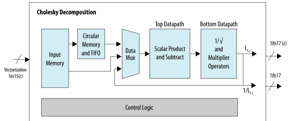
Figure 69. Cholesky Decomposition Top-level Design
