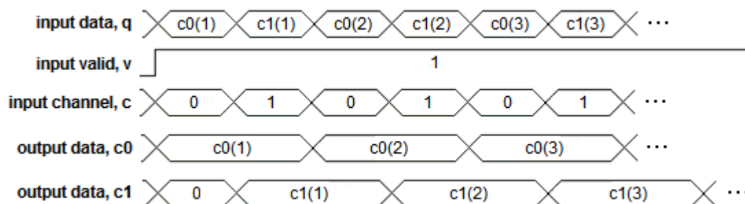
Figure 89. Channel Viewer Output for Two Channels on a Single Wire
