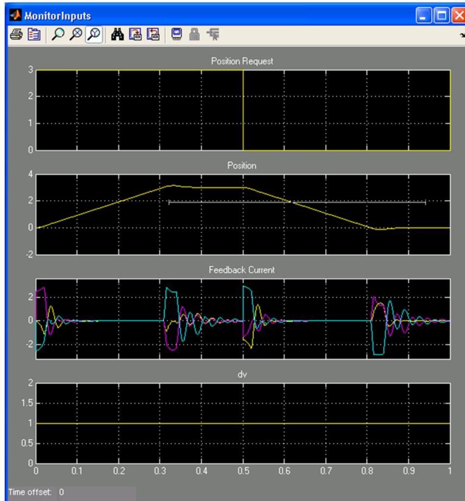
Figure 49. Input Position Request
