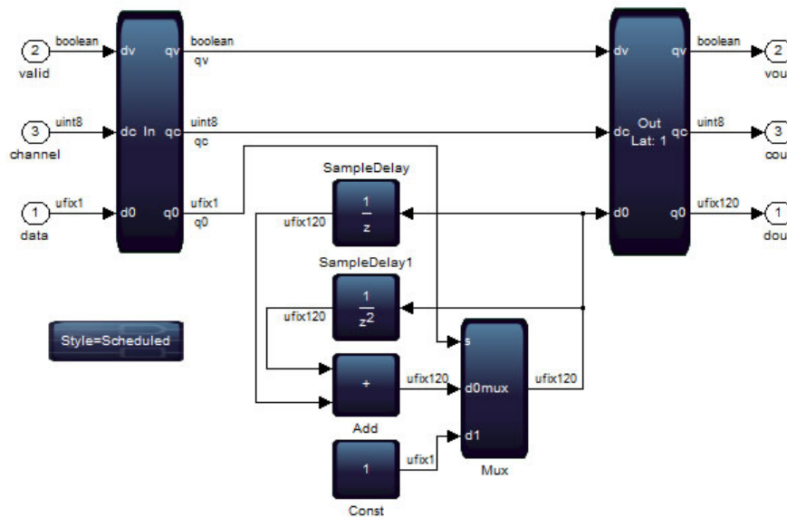
Figure 32. Updated Fibonacci Subsystem
