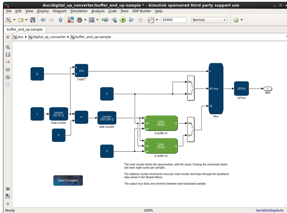
Figure 54. Buffer and Up-Sample
