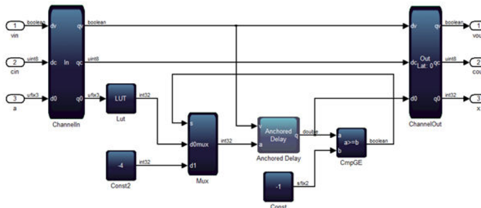
Figure 78. SampleDelay Block Example 2
