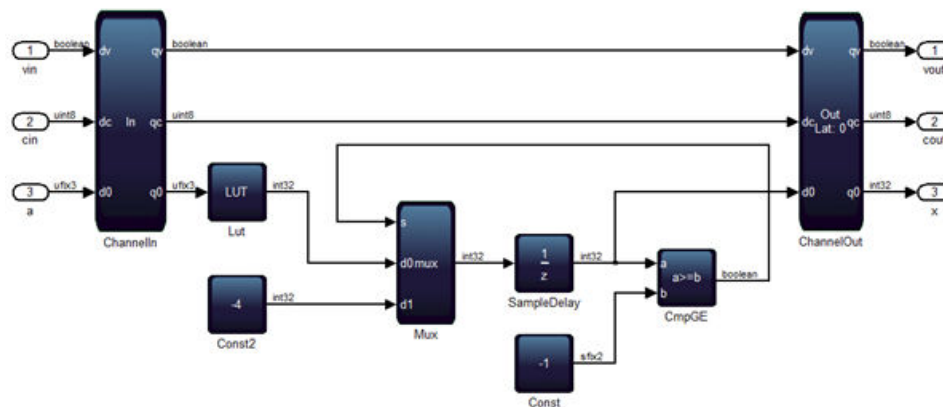
Figure 77. SampleDelay Block Example
