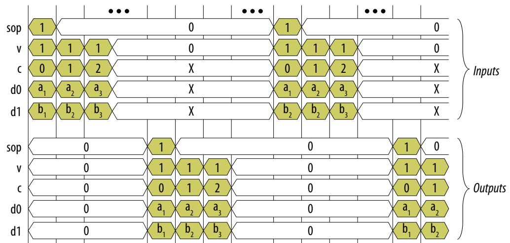
Figure 84. Multichannel Clock Rate Simulation with no Register Outputs
