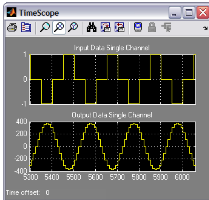
Figure 93. Interpolate by 5 Filter Increasing Sample Rate of a Sine Wave Input
