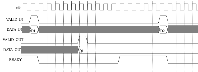
Figure 86. Ready Signal Timing
