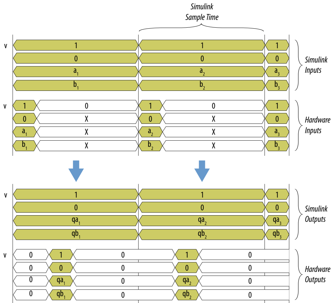
Figure 80. Single Channel Data Rate Simulation with no Register Outputs
