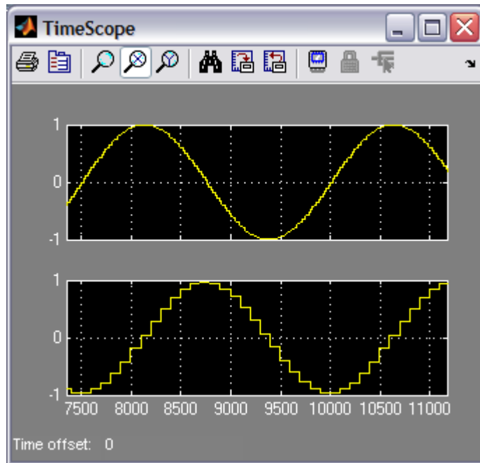
Figure 91. Decimating by 5 Filter Decreasing Sample Rate of a Sine Wave Input
