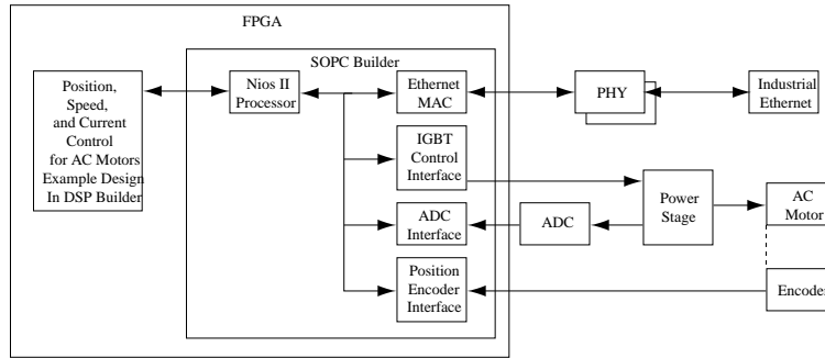
Figure 48. AC Motor Control System Block Diagram
