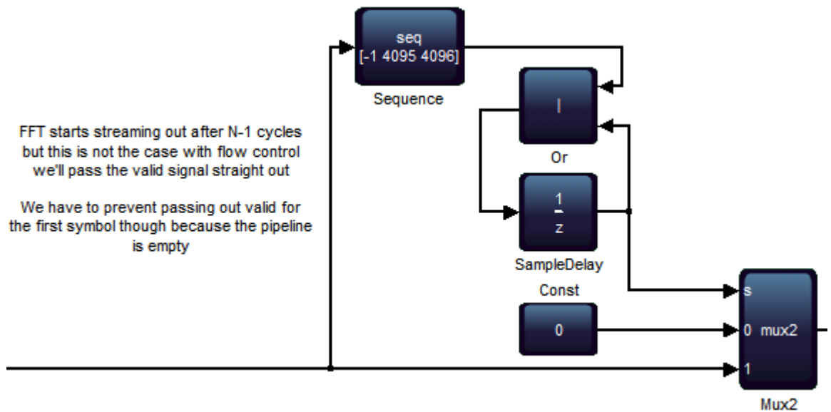
Figure 74. Sequence Block in the 4K FFT Design Example
