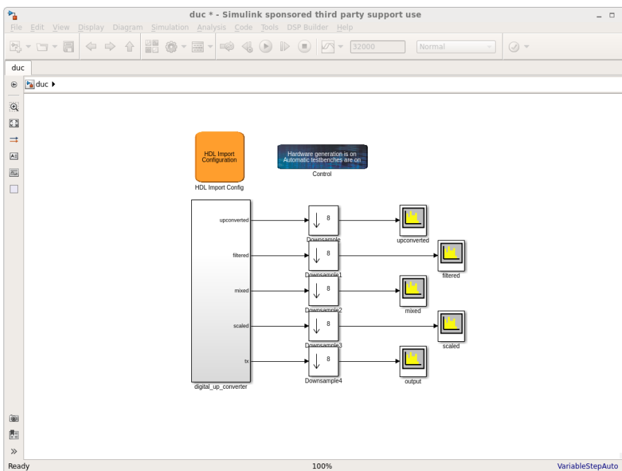
Figure 63. Top-level Design with HDL Import Config Block
