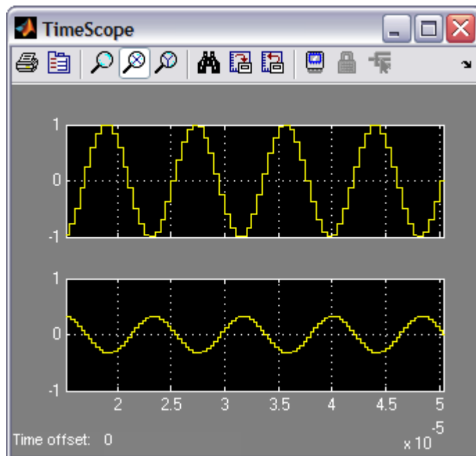
Figure 92. Sample Rate of a Sine Wave Input Interpolated by 3 and Decimated by 2
