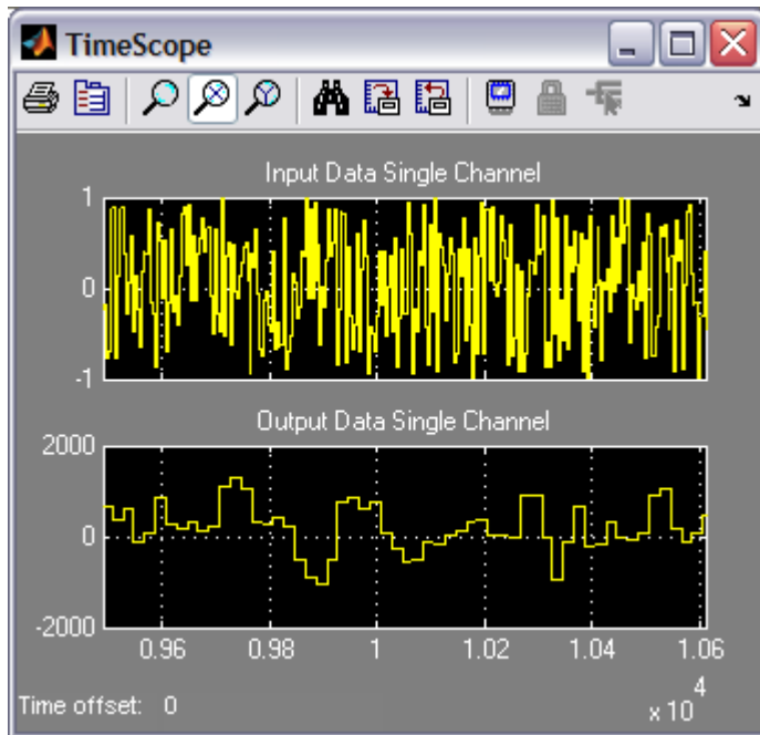
Figure 90. Decimate by 5 Filter Decreasing Sample Rate of a Random Noise Input
