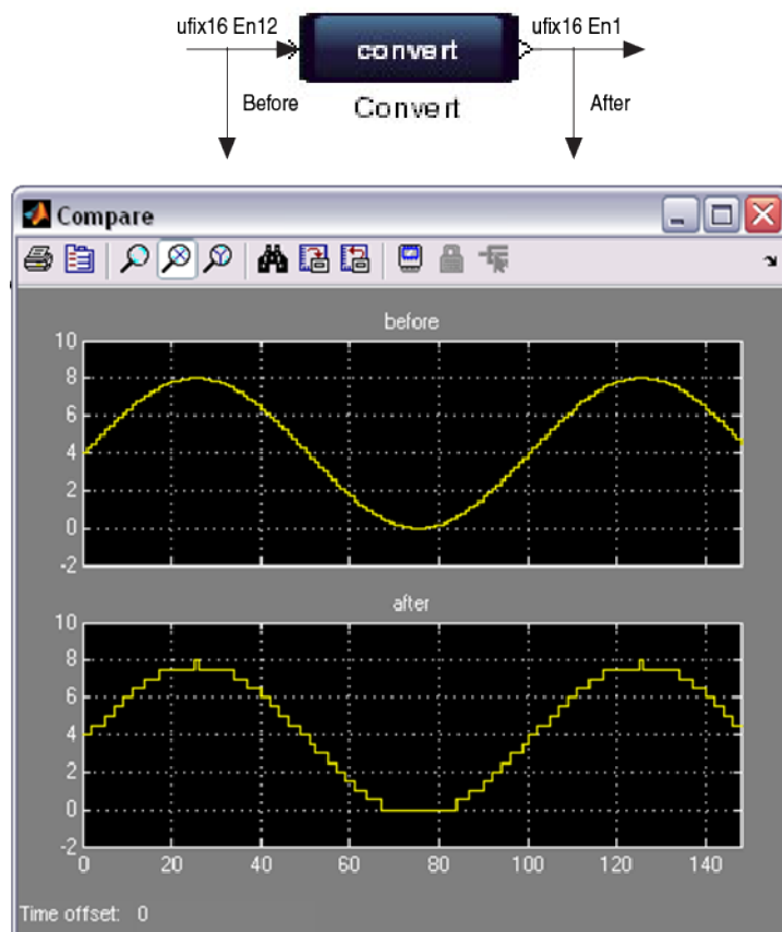
Figure 22. Convert Block Using Same Number of Bits while preserving real-world value
