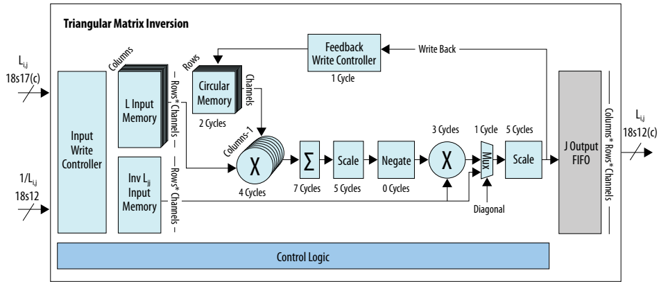
Figure 70. Triangular Matrix Inversion Top-level Design
