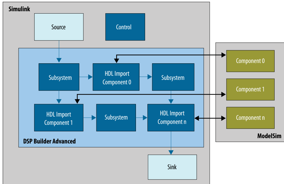
Figure 79. HDL Import Block Placement
