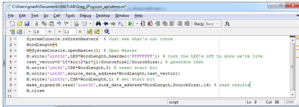
Figure 29. MATLAB API
