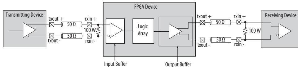
Figure 73. LVDS Interface with External Resistor Network on the Top and Bottom I/O Banks
