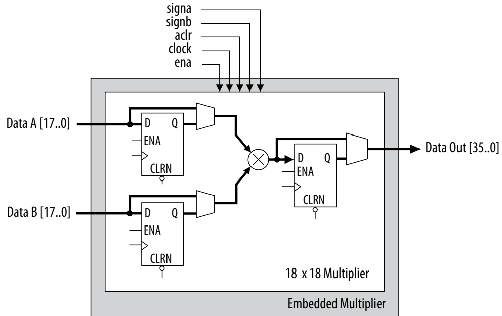
Figure 35. 18-Bit Multiplier Mode
