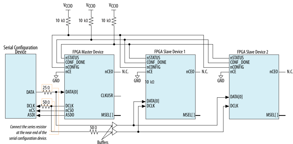
Figure 86. Devices Receiving the Same Data with a Single .sof File in Multi-Device AS Configuration
