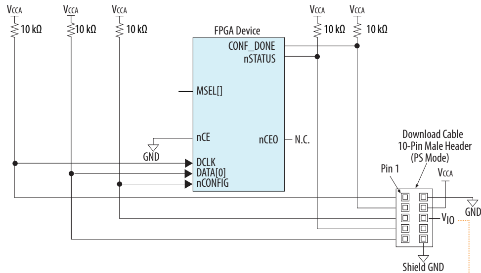
Figure 91. Single Device PS Configuration Using an Intel Download Cable
