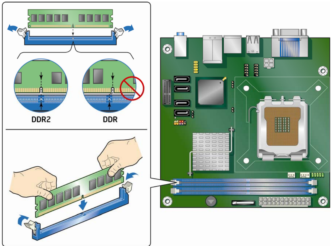
Figure 16. Installing a DIMM
