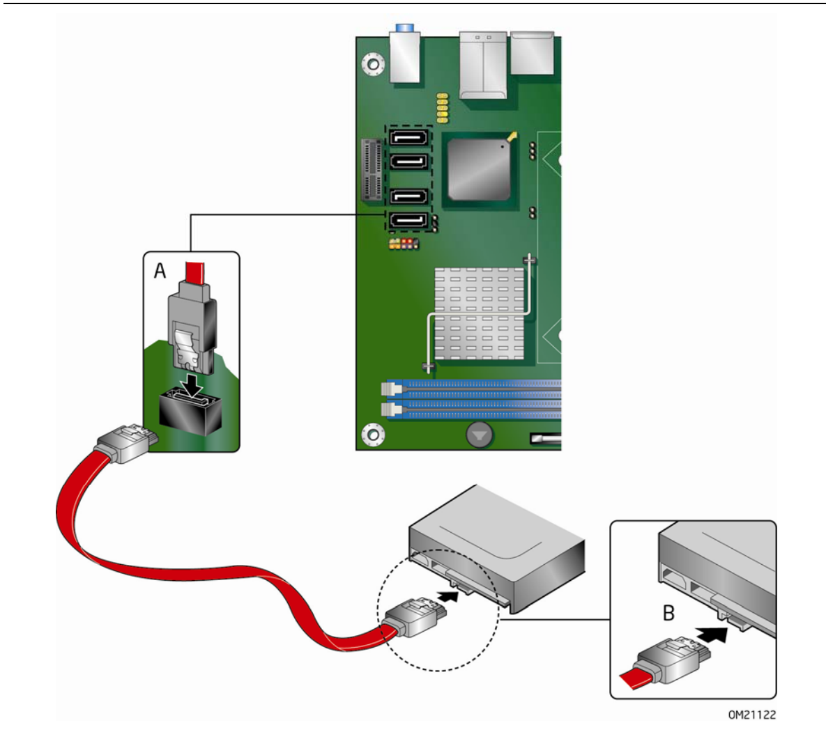
Figure 17. Connecting a Serial ATA Cable
