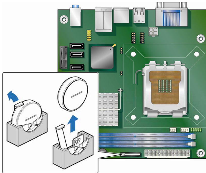
Figure 23. Removing the Battery
