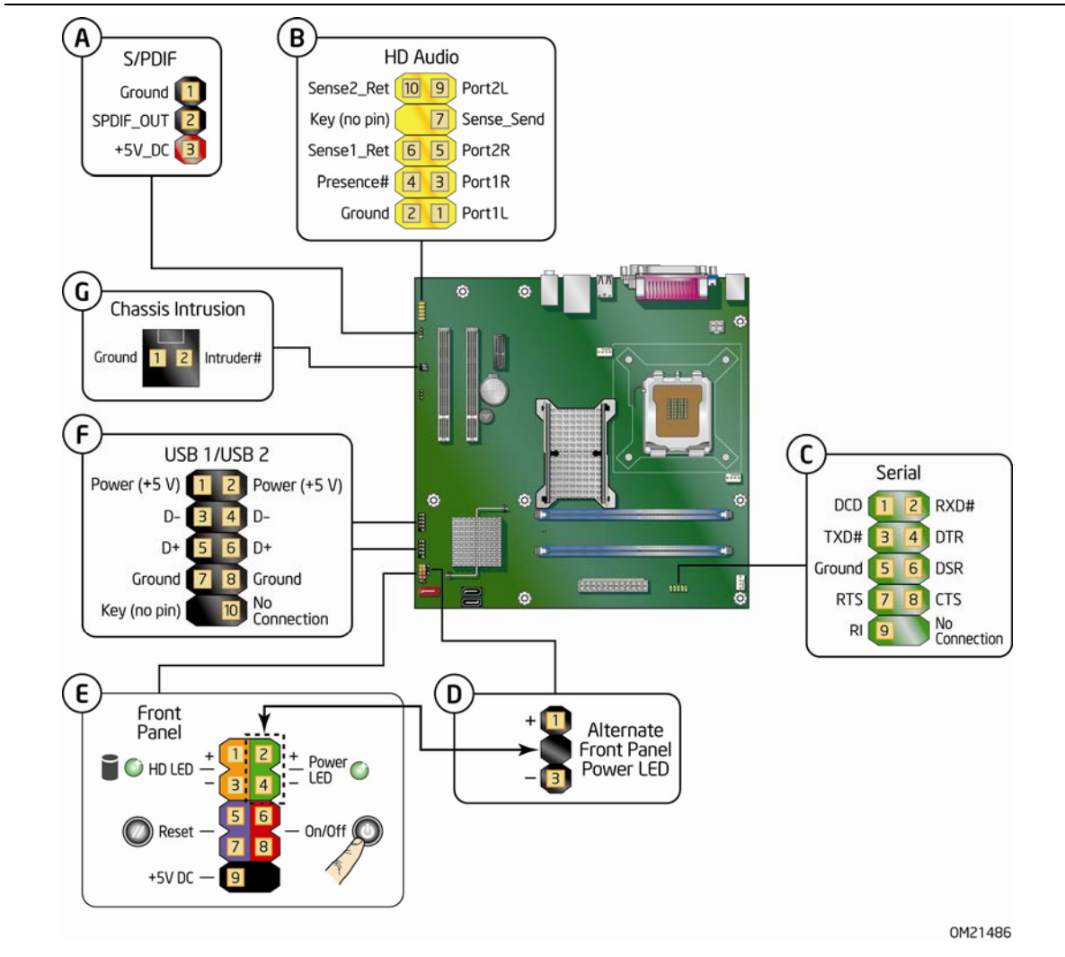
Figure 18. Internal Headers
