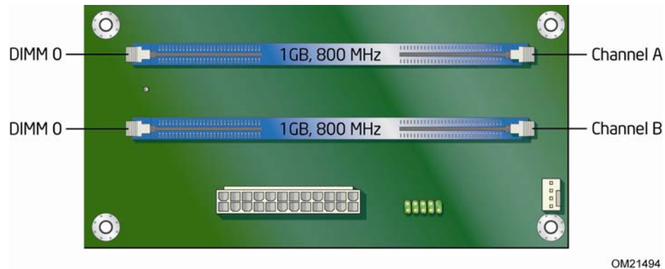
Figure 14. Dual Channel Memory Configuration Example
