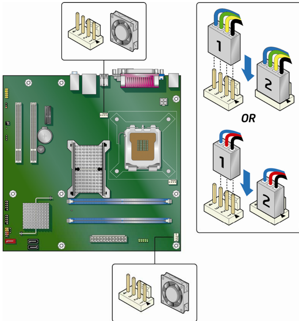
Figure 20. Location of the Chassis Fan Headers
