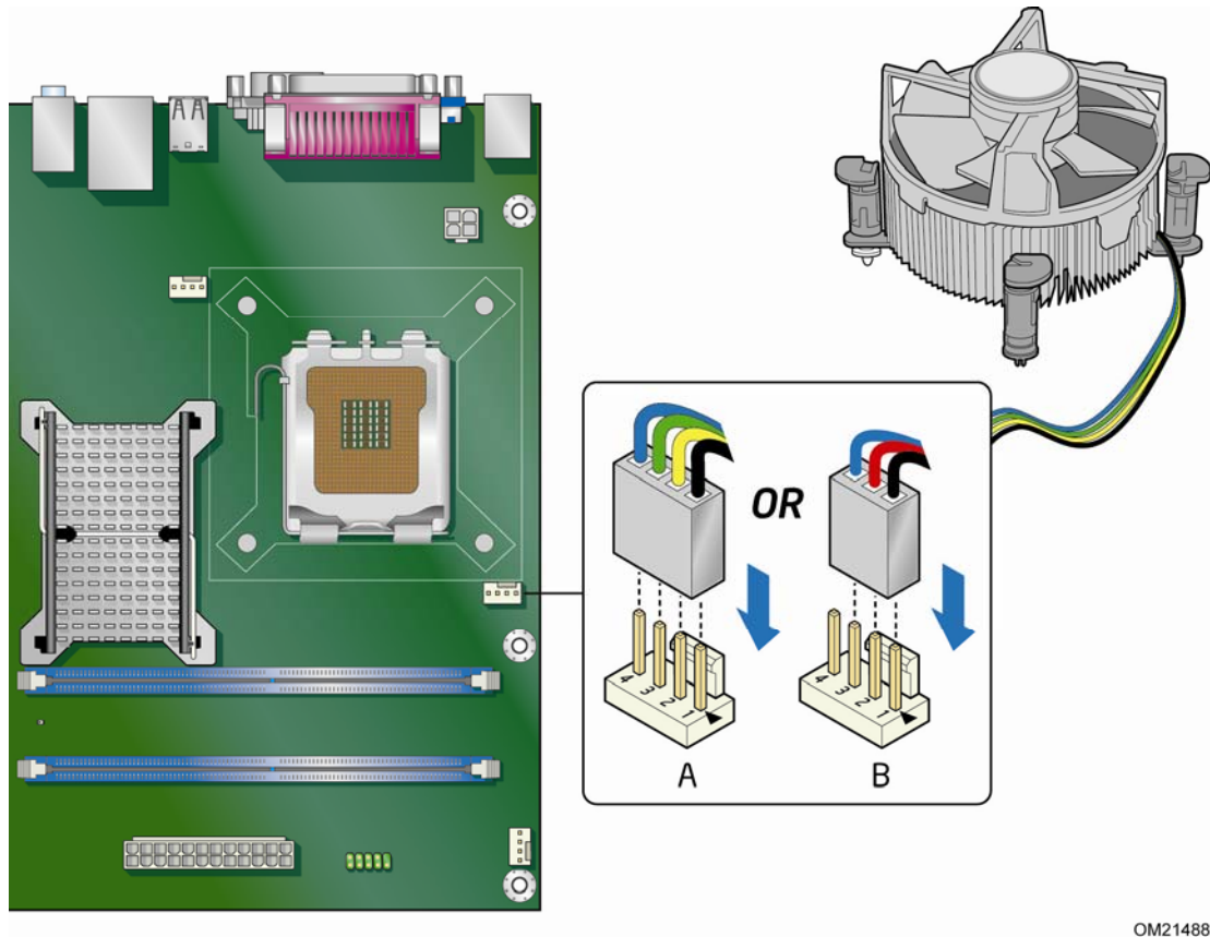
Figure 13. Connecting the Processor Fan Heat Sink Cable
