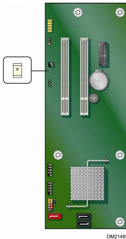
Figure 4. Location of the +5 V Standby Power Indicator
