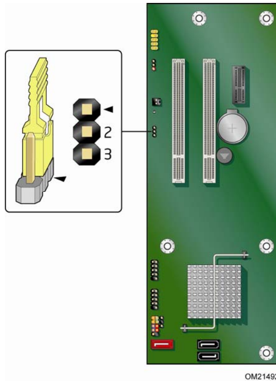
Figure 22. Location of the BIOS Configuration Jumper Block
