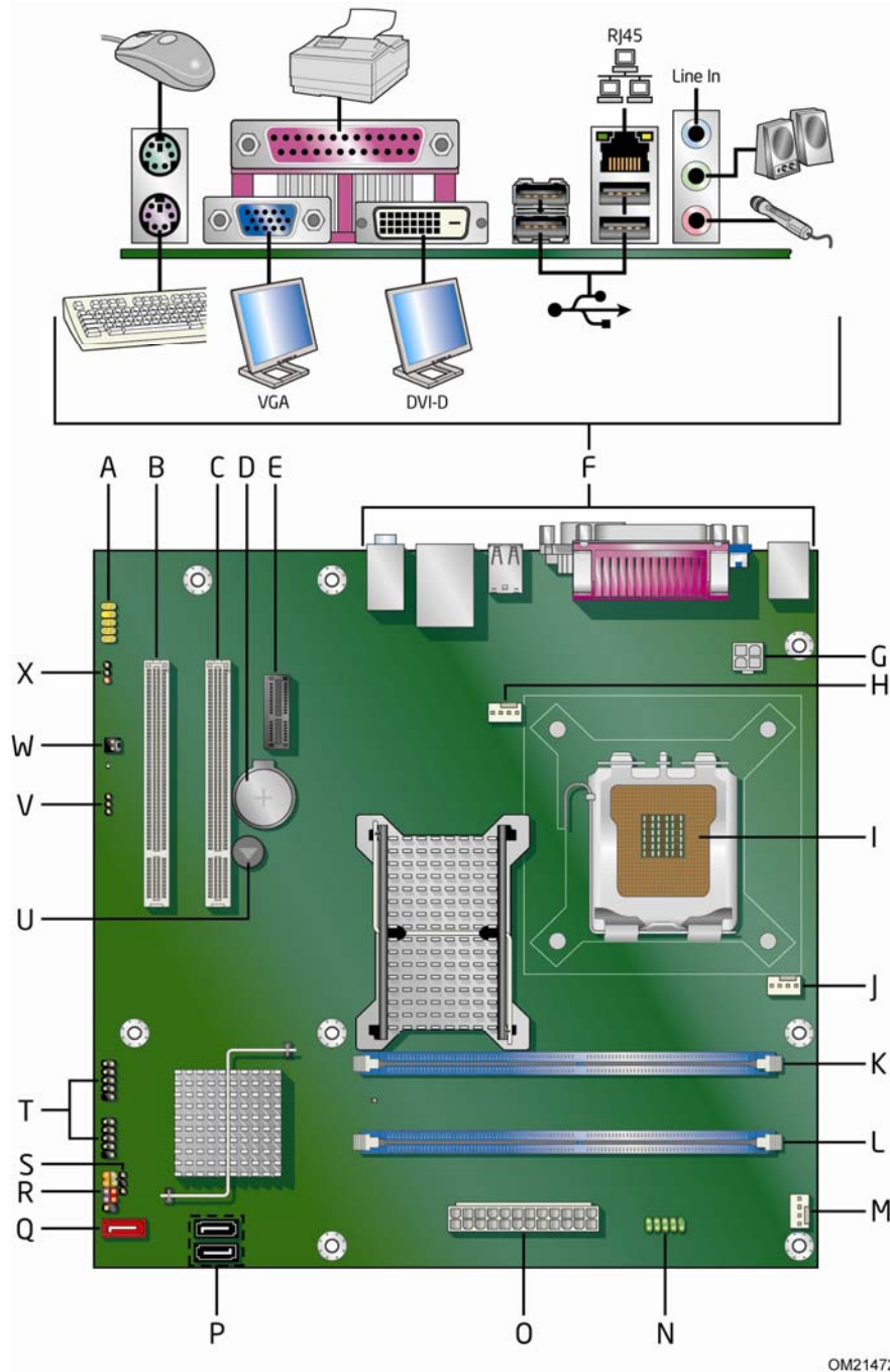
Figure 1. Intel Desktop Board DQ43AP Components
