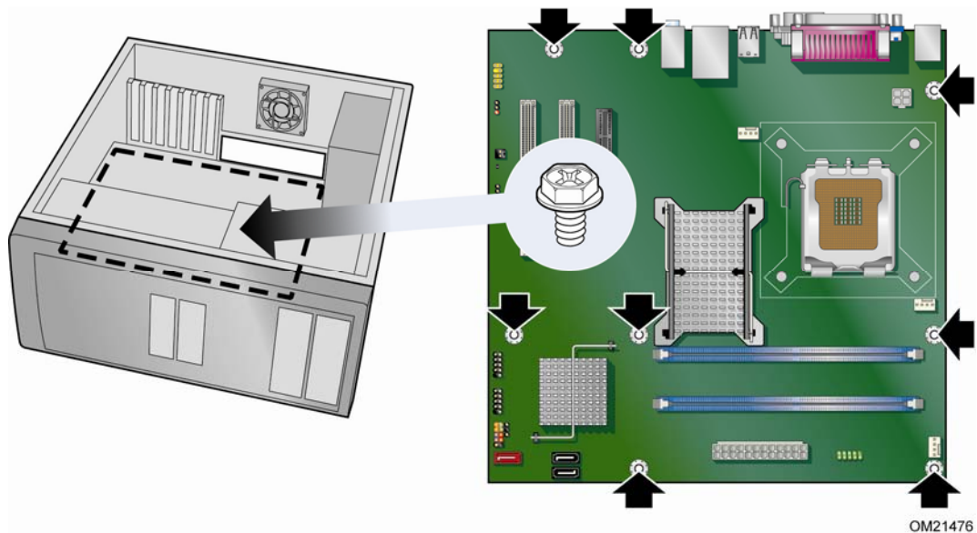
Figure 6. Intel Desktop Board DQ43AP Mounting Screw Hole Locations
