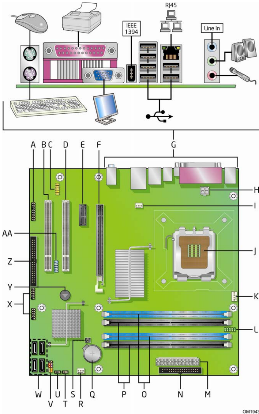
Figure 1. Desktop Board DG965SS Components
