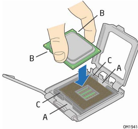
Figure 10. Install Processor
