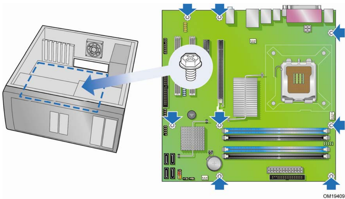
Figure 5. Desktop Board DG965SS Mounting Screw Hole Locations
