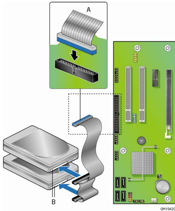
Figure 20. Connecting the IDE Cable
