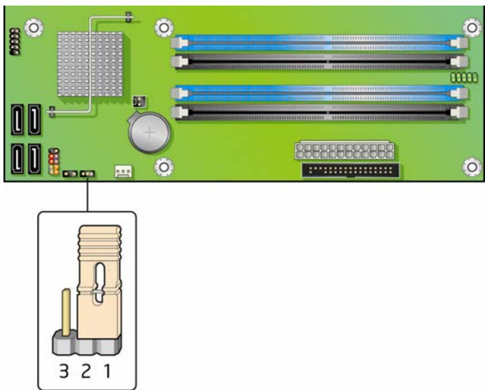
Figure 27. Location of the BIOS Configuration Jumper Block
