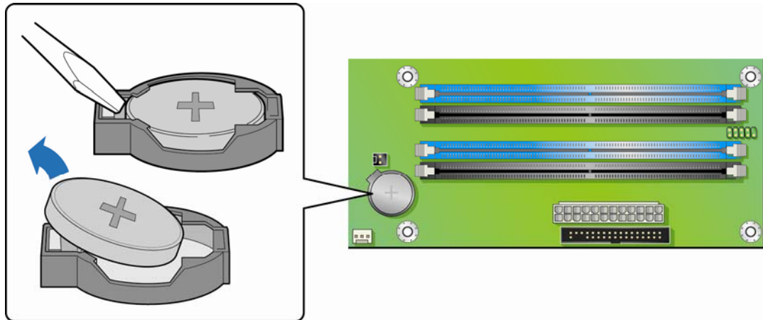
Figure 29. Removing the Battery
