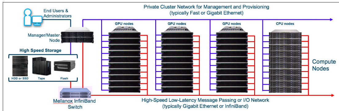
Figure 7-6 IBM PowerAI V1.5 integrated with Deep Learning Impact and IBM Spectrum Conductor with Spark in a high-performance computing environment
