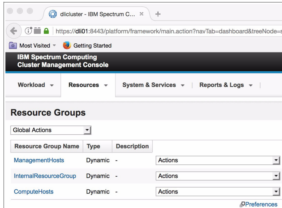
Figure 6-17 Resource group configuration window
