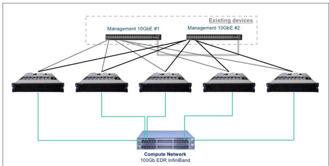
Figure 7-4 Network configuration image for the NVIDIA-Docker case
