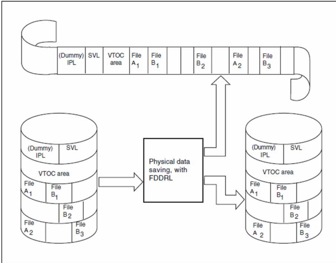
Figure 3: Physical data saving
