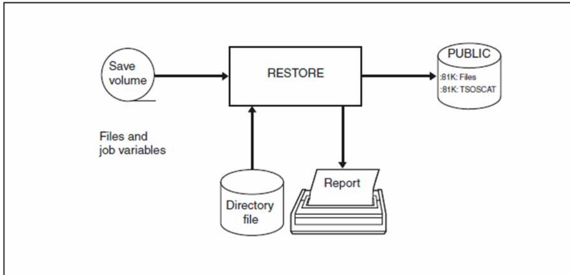
Figure 10: Restoration to other pubsets
