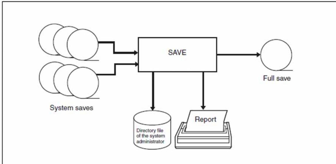
Figure 19: Creating a complete system save
