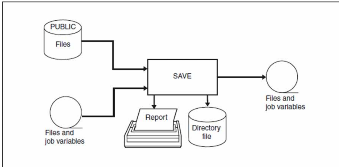
Figure 16: Merging save data
