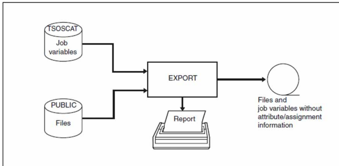
Figure 14: Exporting files without attribute and assignment information
