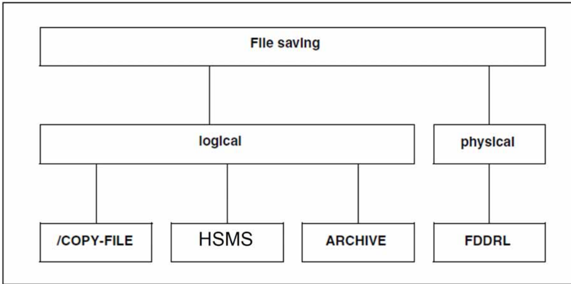
Figure 1: Data saving in BS2000 OSD/BC
