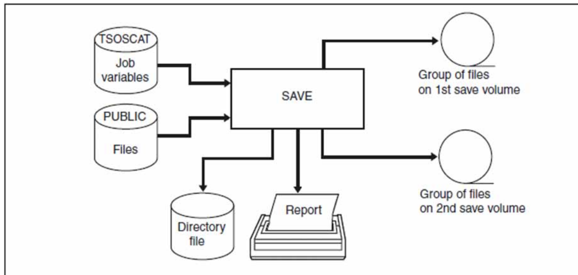
Figure 15: Save, parallel processing
