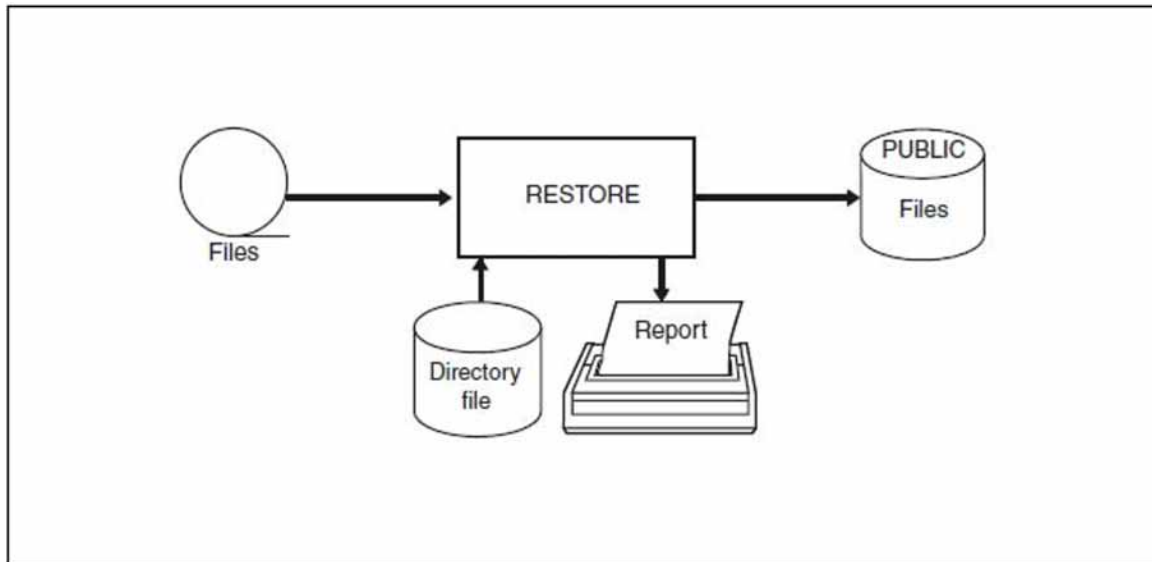
Figure 8: Restoration with the directory file
