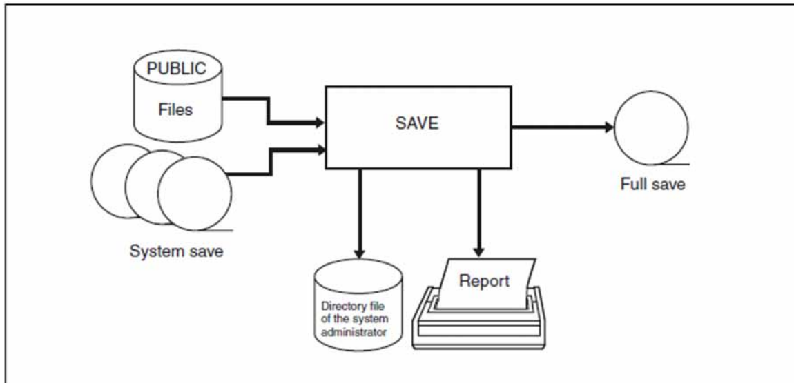
Figure 18: Restoration from system save
