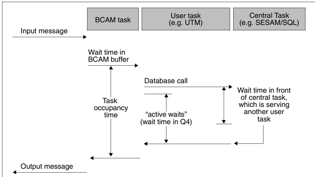
Figure 18: Time behavior of multi-level task concepts
