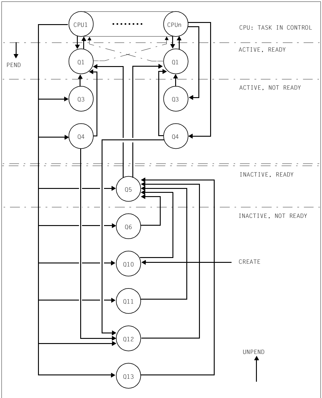
Figure 7: Queue transfers
