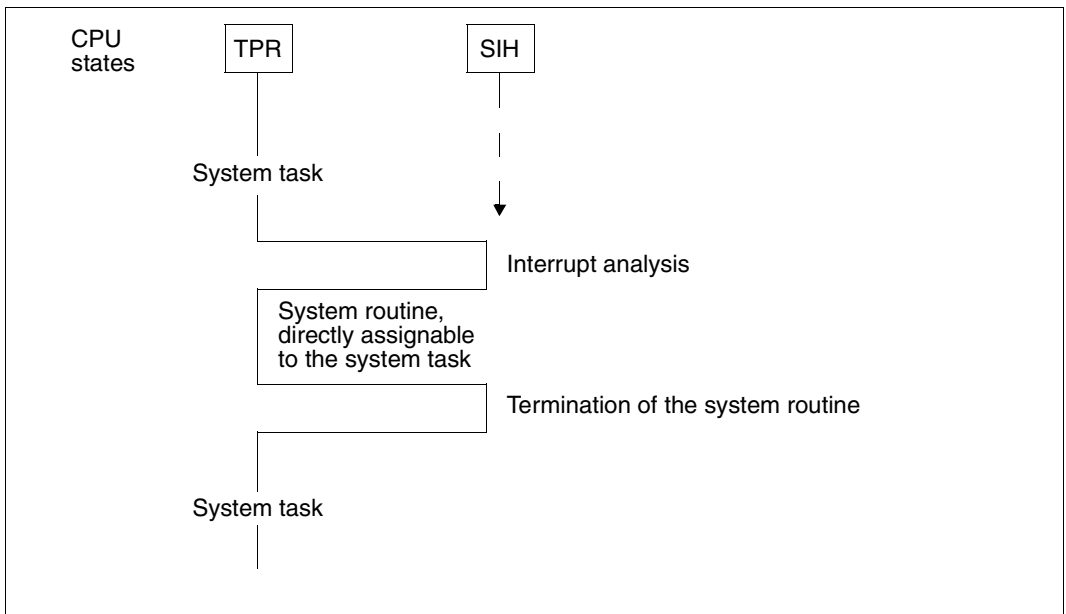
Figure 6: BS2000 CPU states (system task)
