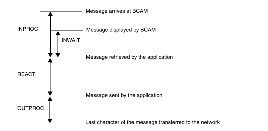
Figure 15: BCAM times
