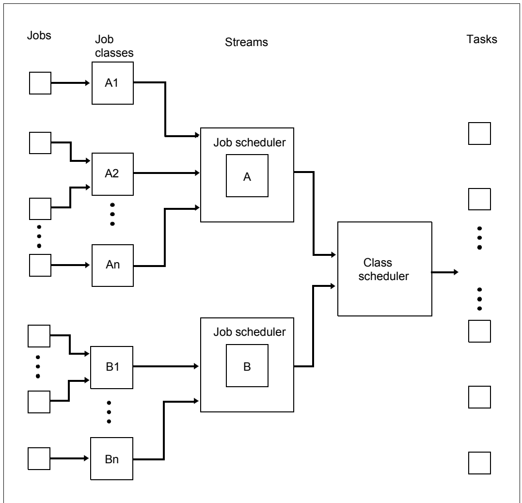
Figure 17: Job management components
