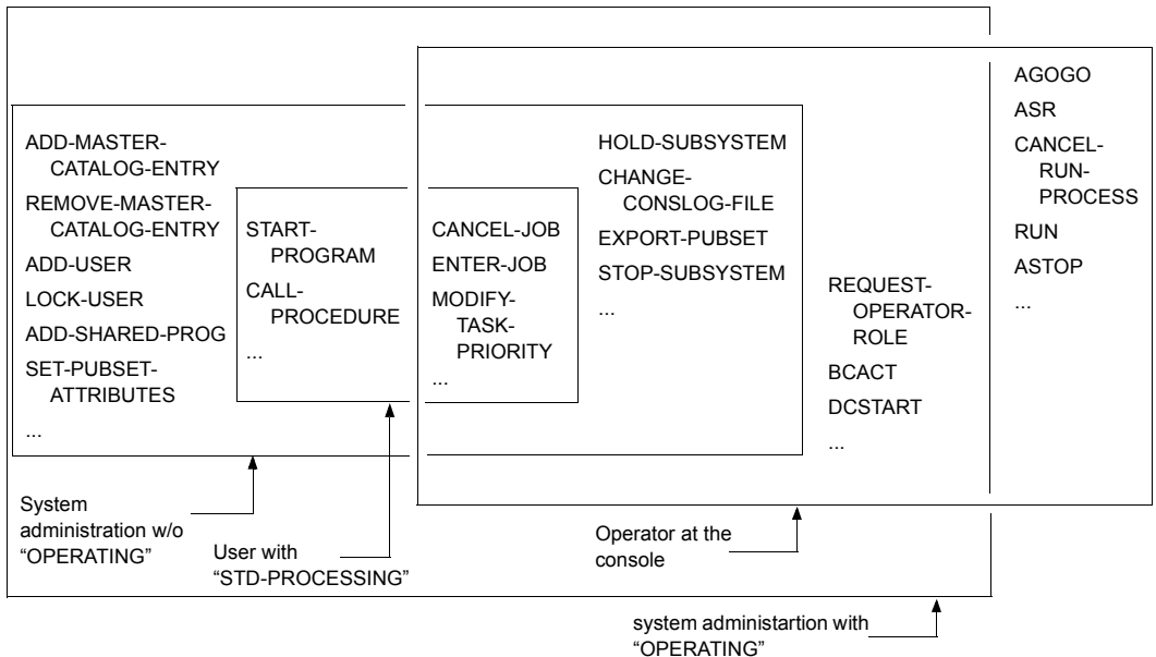
Figure 20: Authorization to enter commands
