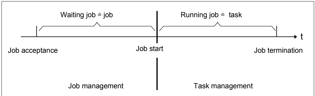
Figure 16: Relationship of job and task
