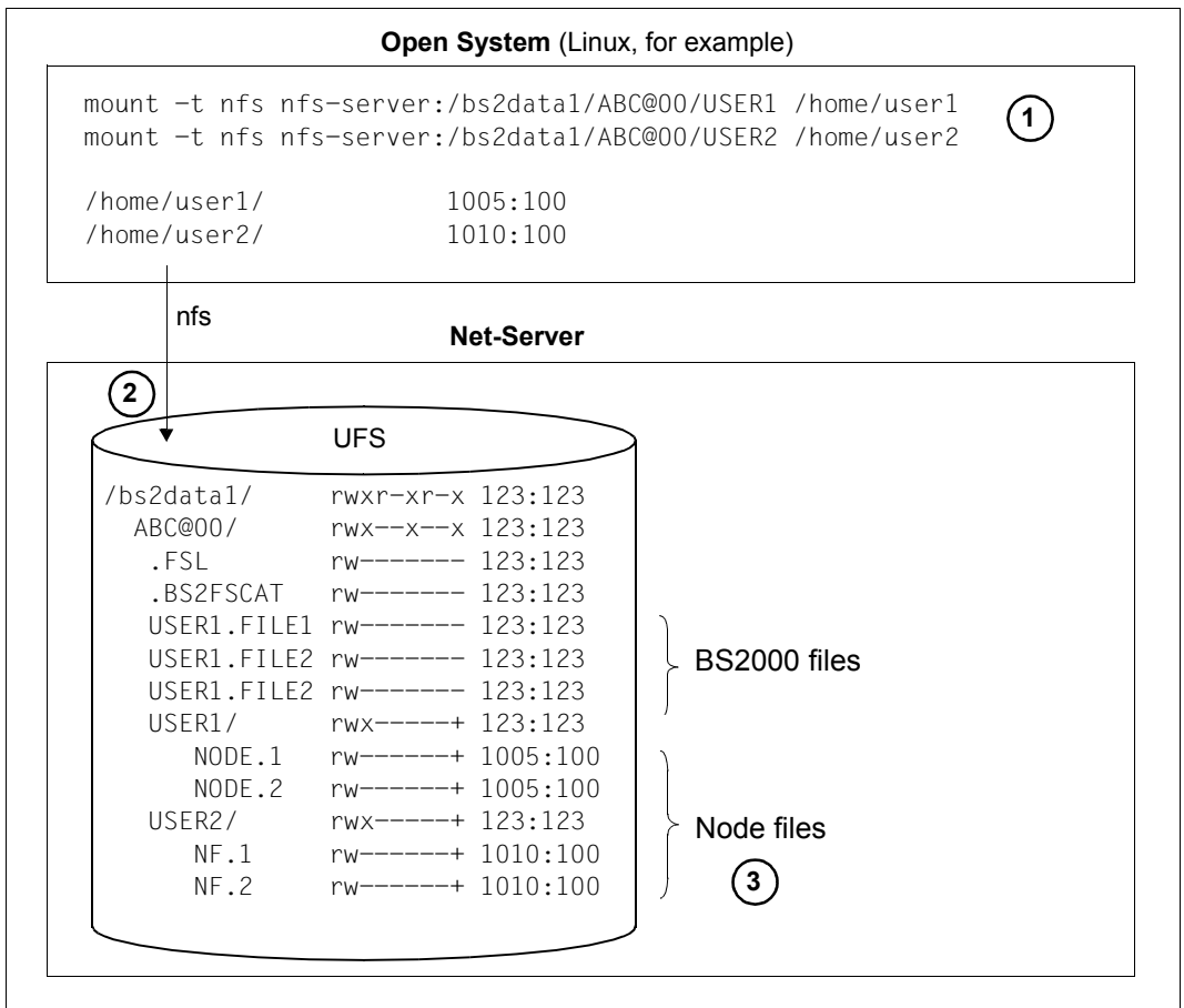
Figure 15: Access of open systems to Net-Storage
