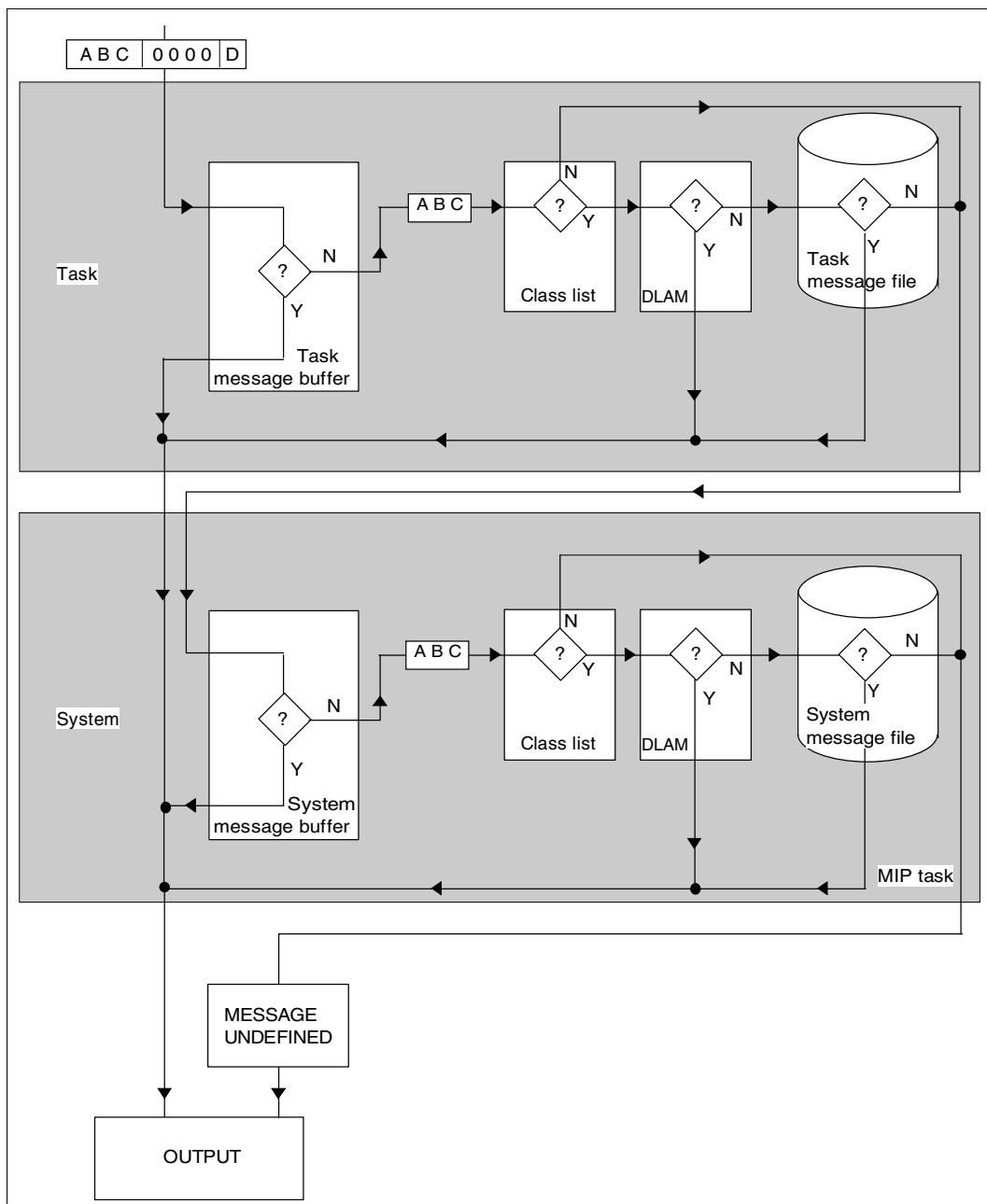
Figure 23: Message search in BS2000
