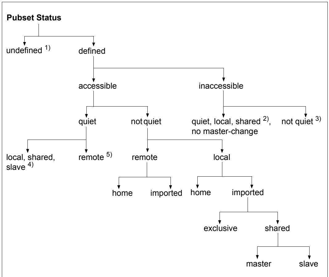
Figure 13: Static pubset states
