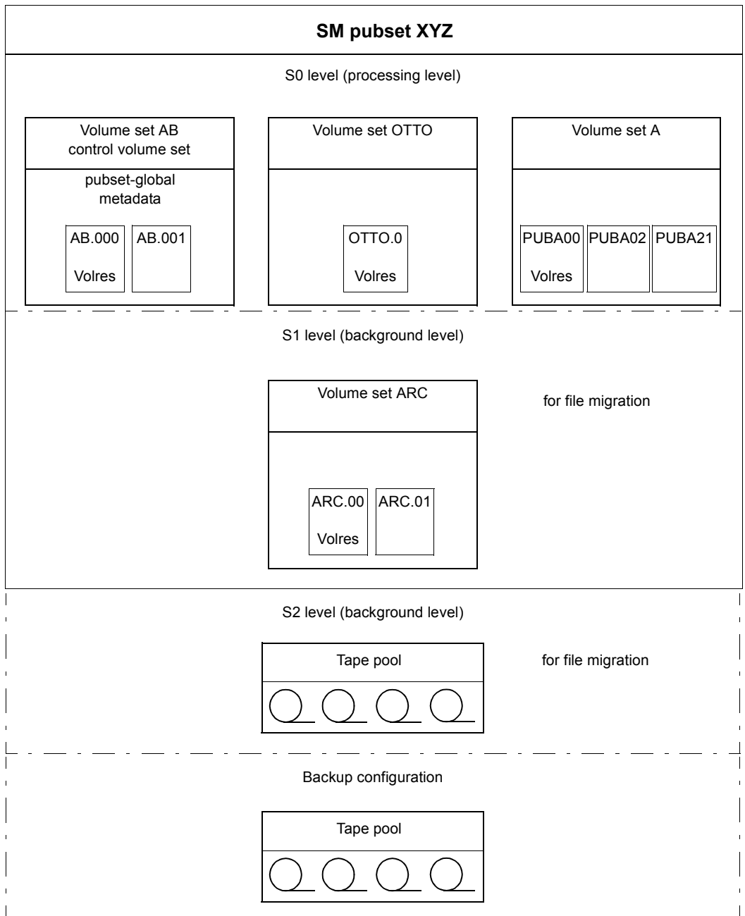
Figure 9: SM pubset structure with HSMS configuration
