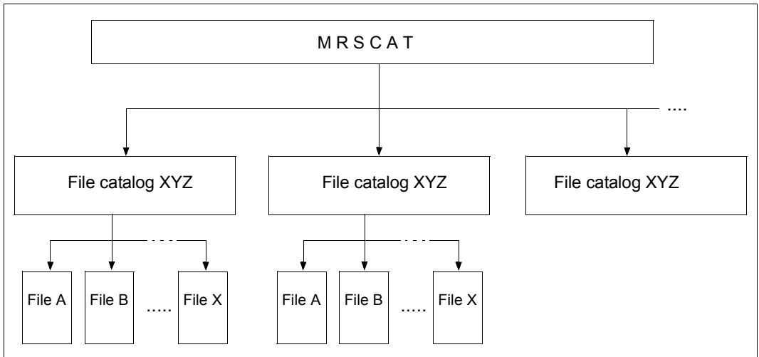
Figure 10: MRSCAT catalog structure - file catalog
