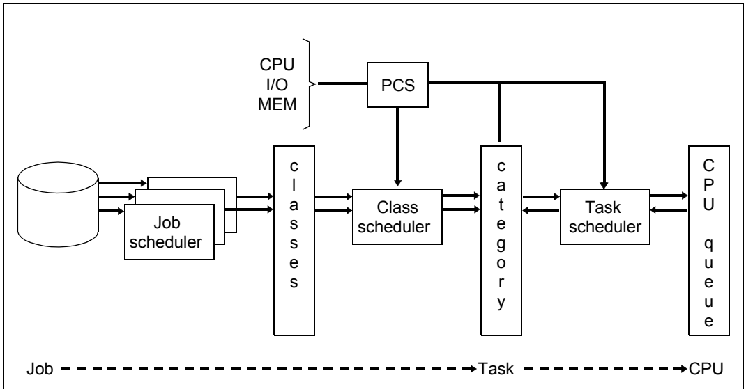
Figure 18: Job management – PCS – Task management
