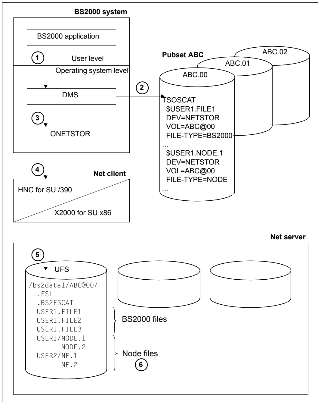
Figure 14: BS2000 access to Net-Storage
