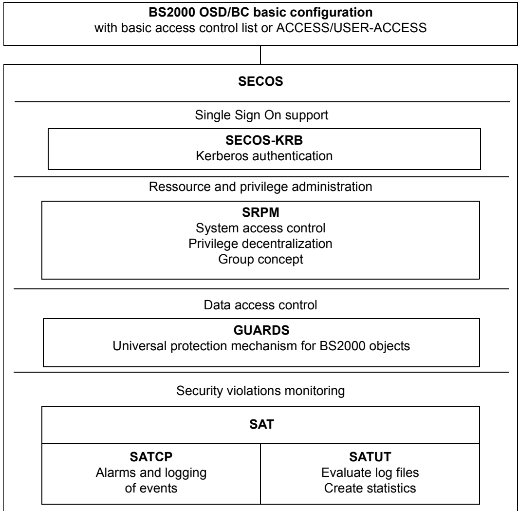
Figure 21: Functional units in the security package
