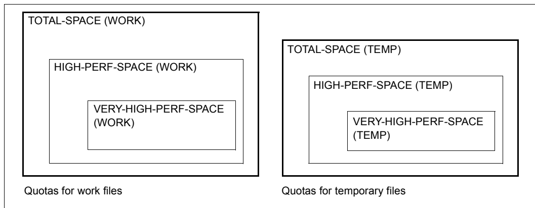
Figure 12: Quota structure for temporary and work files
