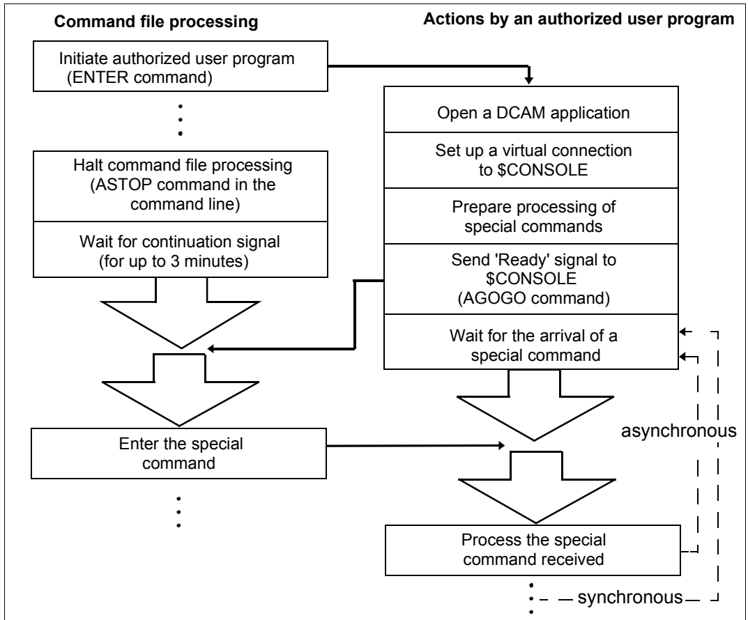
Figure 29: Processing a command file
