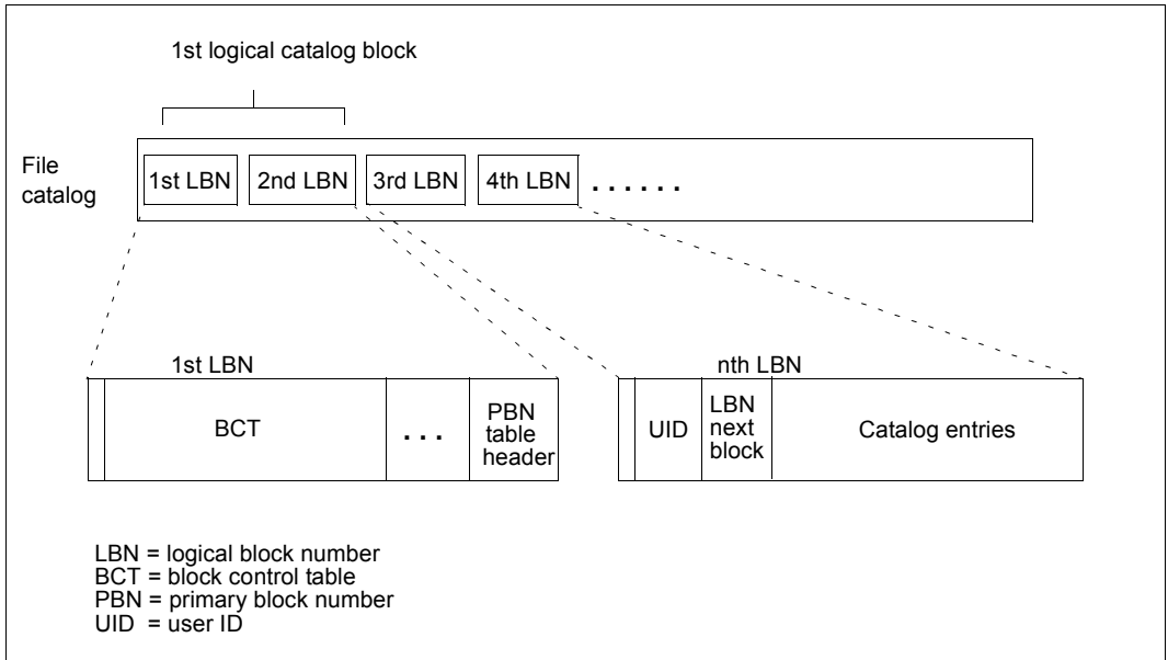
Figure 7: Structure of the file catalog
