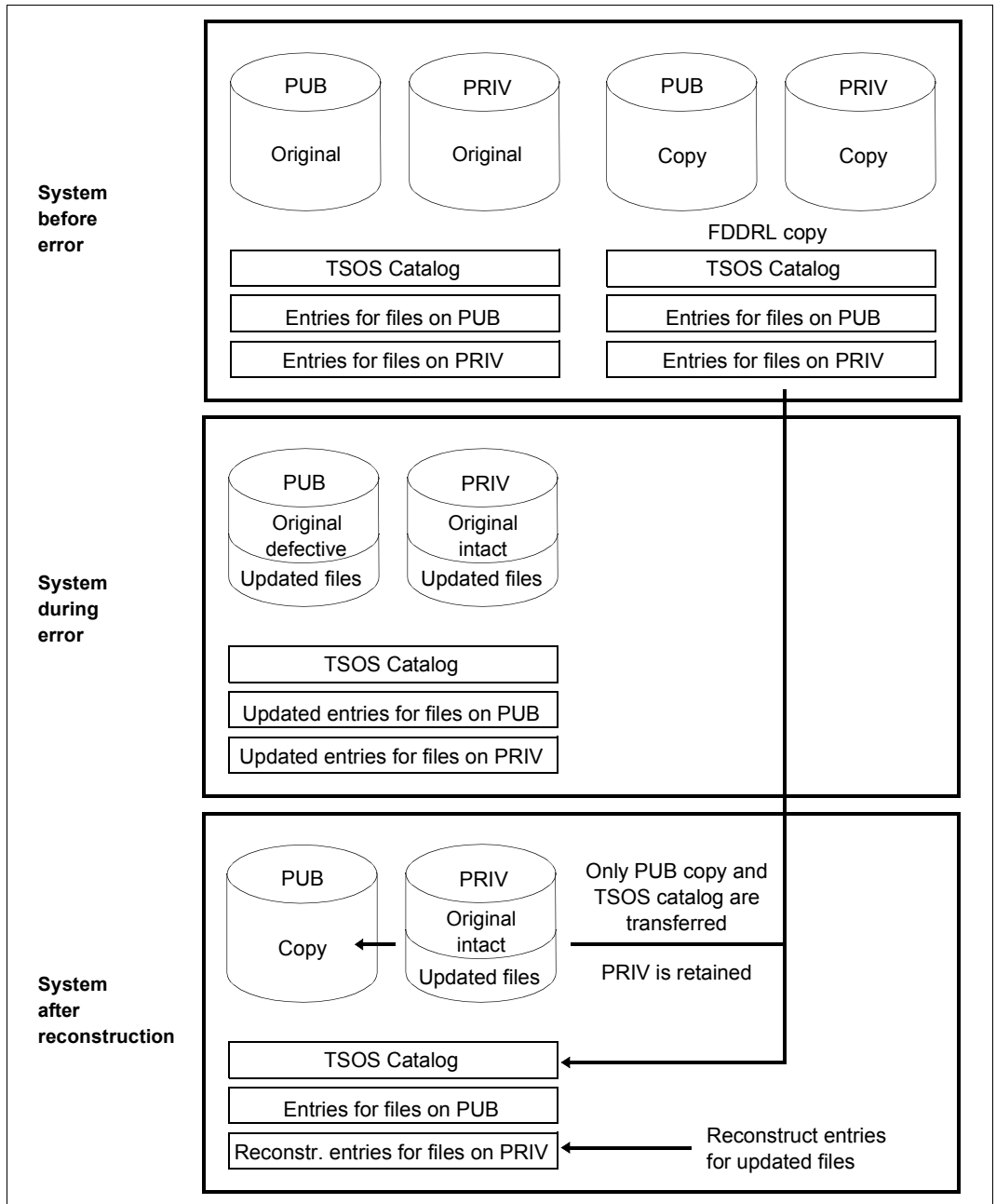
Figure 22: Reconstruction after a system error
