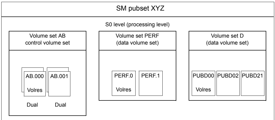
Volume configuration of an SM pubset (example)
