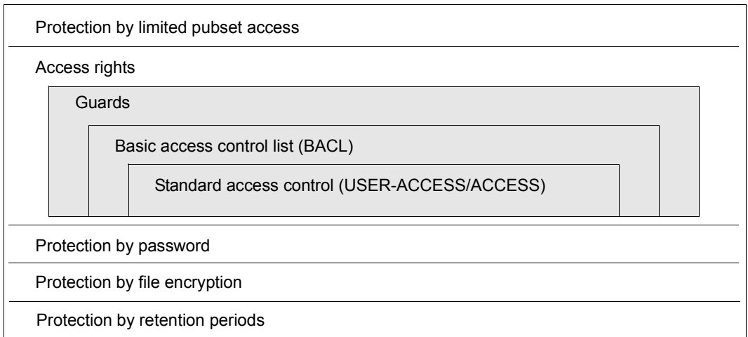
Figure 19: Protection mechanisms for files on a pubset
