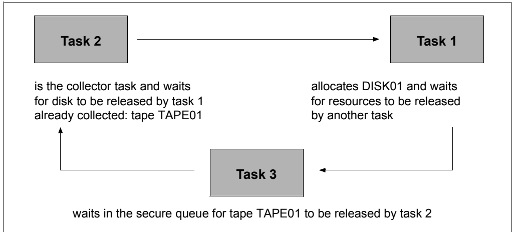
Figure 4: Deadlock situation because of collecting
