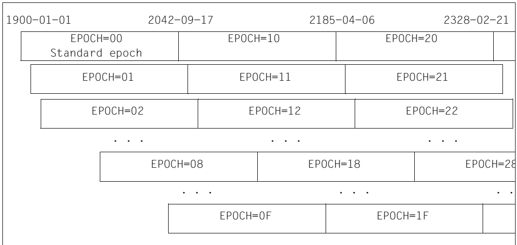
Figure 30: TODR epochs
