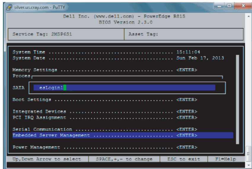
Figure 16. Rack-mount SMW User-defined LCD String Settings
