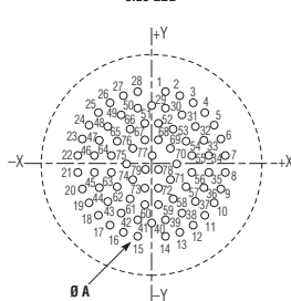
79 contacts size 22D
